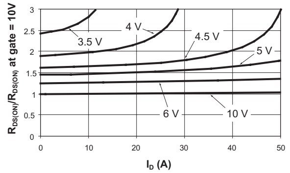
Normalized R_{DS(ON)}
