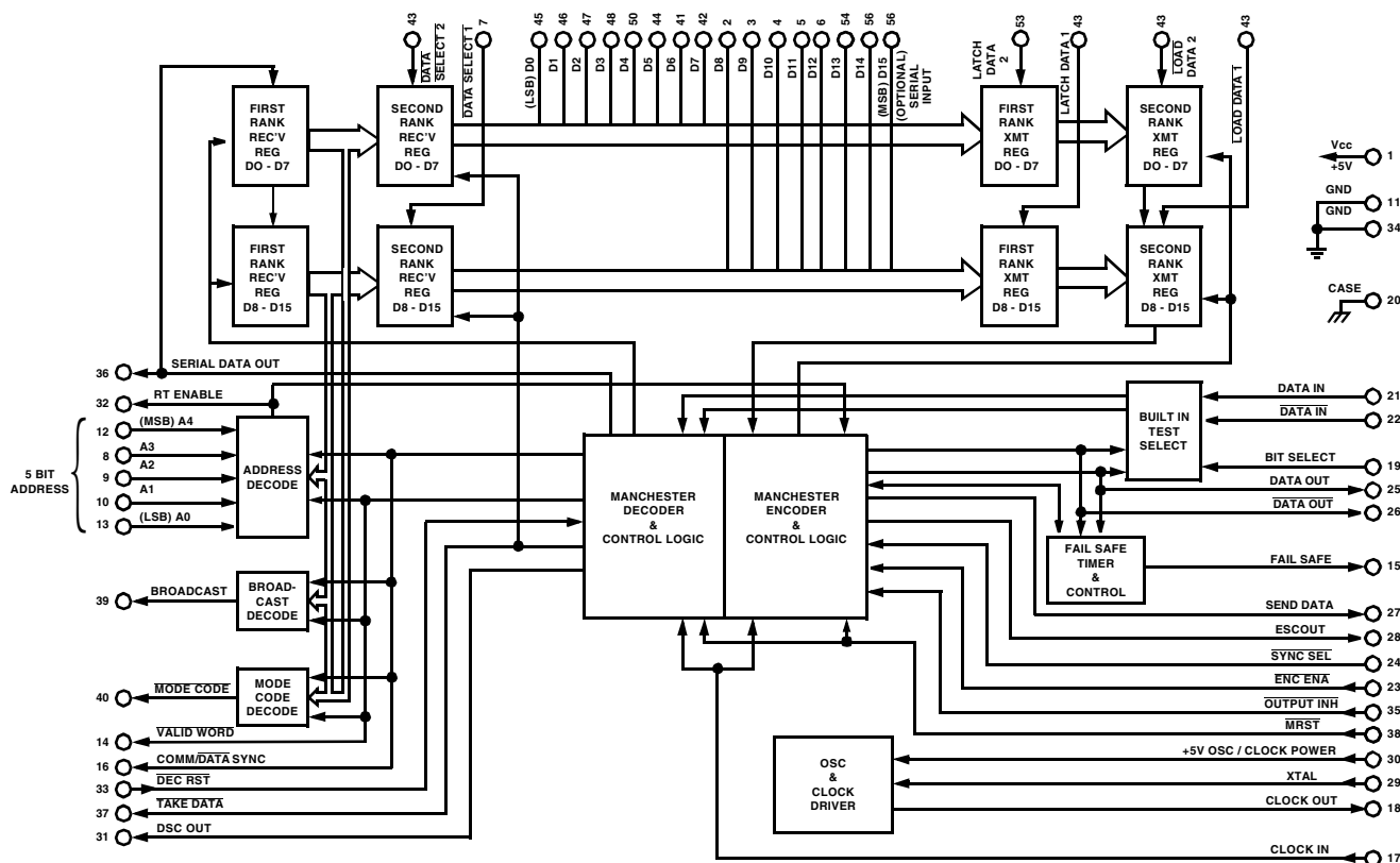
Figure 1 – Functional Diagram
