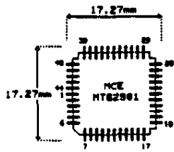
44 PIN J-LEAD PACKAGE TOP VIEW
