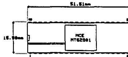
40 PIN DIL CERAMIC PACKAGE TOP VIEW
