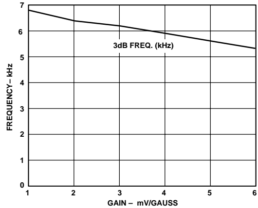
Figure 13. Small-Signal Gain Bandwidth
