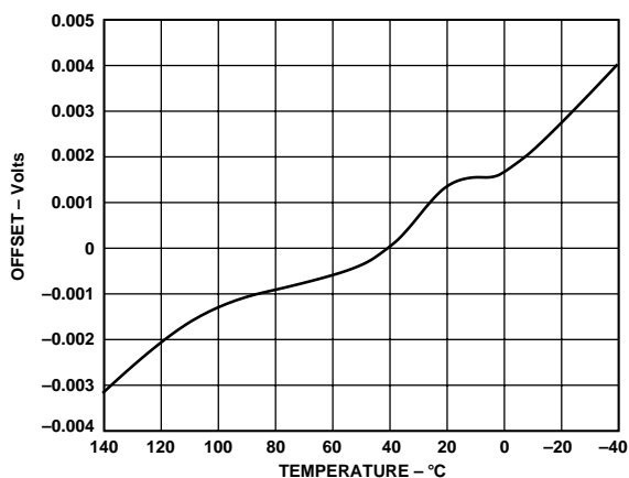
Figure 3. Relative Quiescent Offset vs. Temperature
