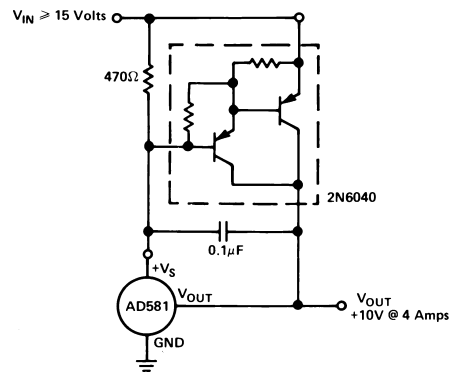
Figure 9. High Current Precision Supply
