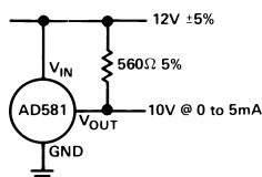
Figure 10. 12-Volt Supply Connection
