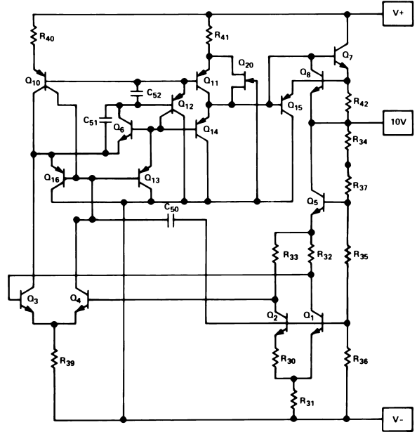
Figure 3. Simplified Schematic
