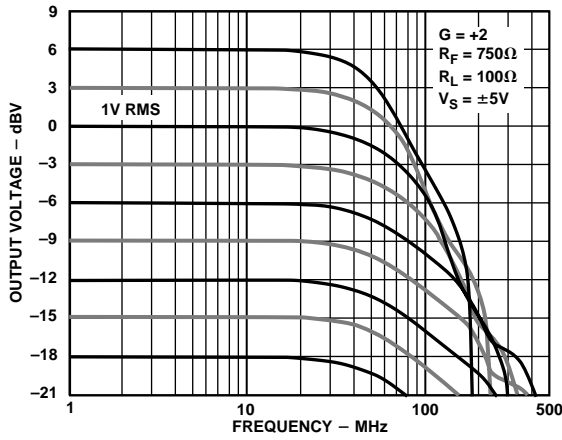
Figure 23. Output Voltage vs. Frequency; V_S = \pm 5V , G = +2 , R_L = 100\Omega
