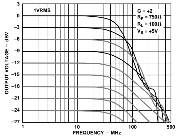
Figure 26. Output Voltage vs. Frequency; V_S = +5V , G = +2 , R_L = 100\Omega
