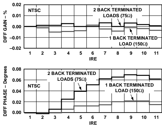
Figure 10. Differential Gain and Differential Phase (per Amplifier)
