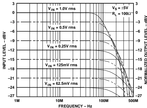
Figure 12. Large Signal Frequency Response
