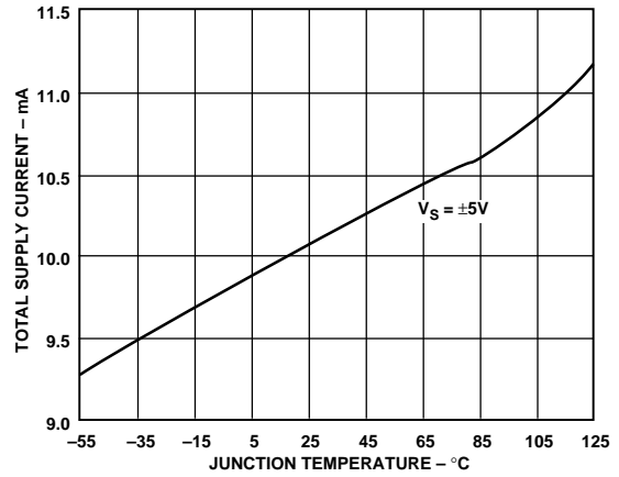
Figure 18. Total Supply Current vs. Temperature
