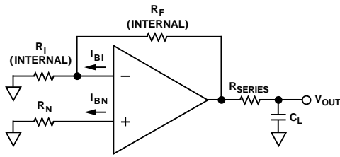
Figure 24. Output Offset Voltage
