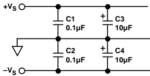
Supply Bypassing
