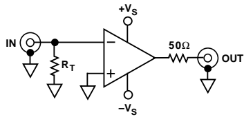
Inverting Configuration
