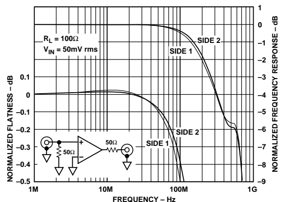
Figure 1. Frequency Response and Flatness
