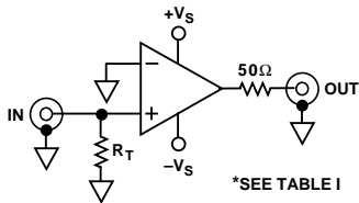
Noninverting Configuration (G = +2)
