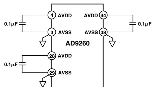
Figure 67. Analog Supply Decoupling
