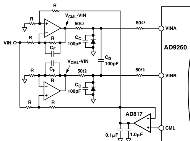
Figure 58. DC-Coupled Differential Driver with Level-Shifting
