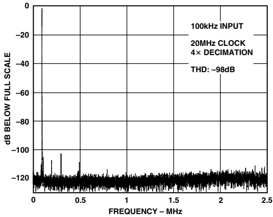
Figure 6. Spectral Plot of the AD9260 at 100 kHz Input, 20 MHz Clock, 4x OSR (5 MHz Output Data Rate)
