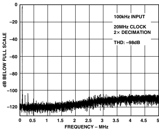
Figure 7. Spectral Plot of the AD9260 at 100 kHz Input, 20 MHz Clock, 2x OSR (10 MHz Output Data Rate)
