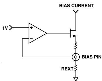
Figure 63. Simplified Bias Pin Circuitry
