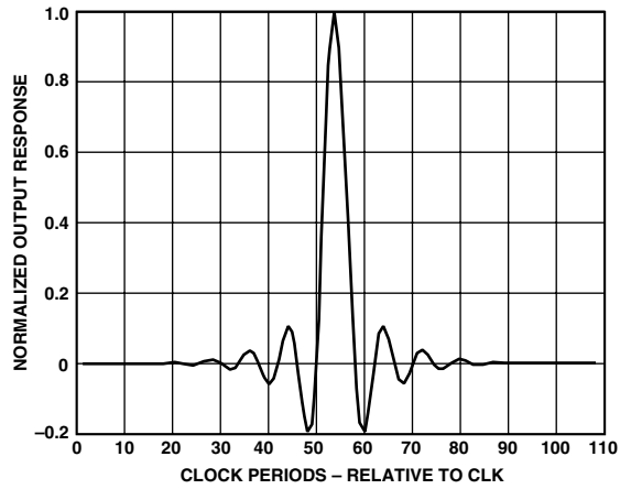
Figure 2b. 4x FIR Filter Impulse Response
