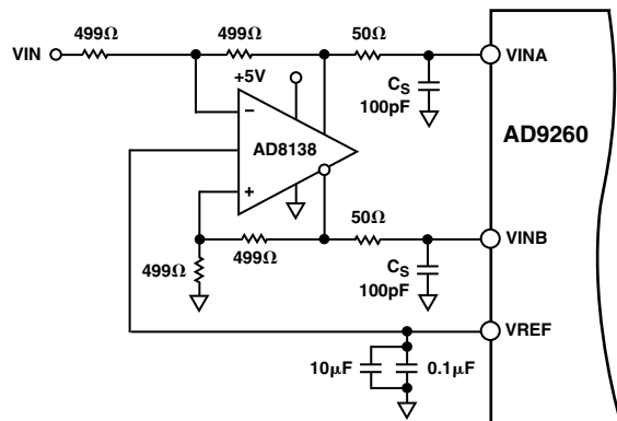
Figure 57. AD8138 Single-Ended Differential ADC Driver
