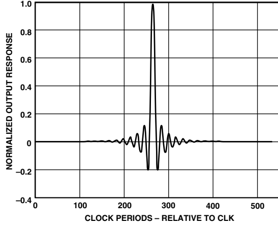
Figure 1b. 8x FIR Filter Impulse Response
