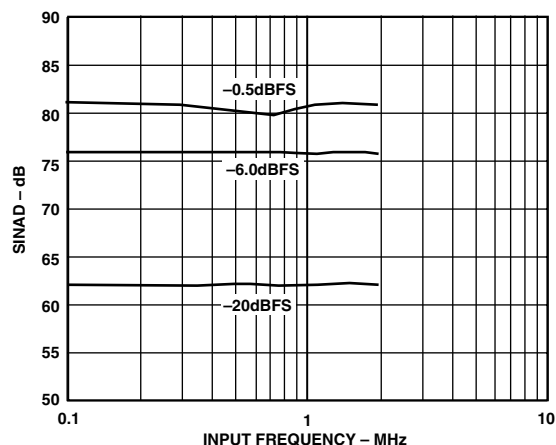
Figure 23. SINAD vs. Input Frequency ( f_{\text{CLOCK}} = 20 \text{ MSPS} )
