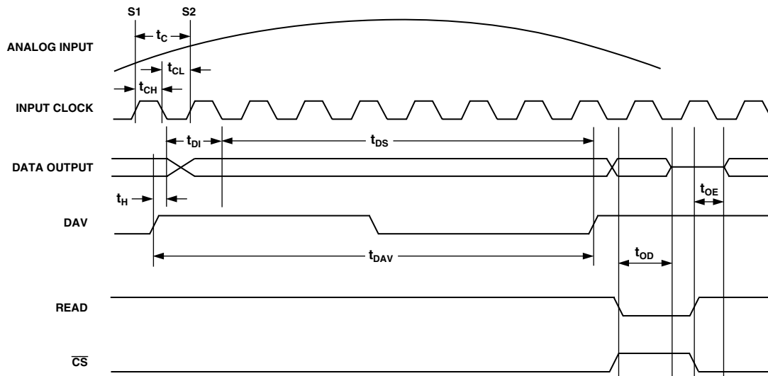
Figure 4a. Timing Diagram
