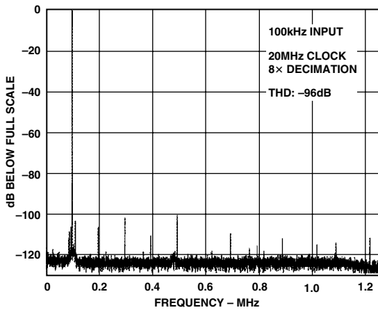
Figure 5. Spectral Plot of the AD9260 at 100 kHz Input, 20 MHz Clock, 8x OSR (2.5 MHz Output Data Rate)
