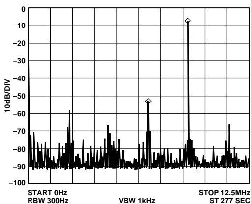
Figure 20. f_{MCLK} = 25 \text{ MHz} , f_{OUT} = 9.1 \text{ MHz} , Frequency Word = 5D2F1AA0
