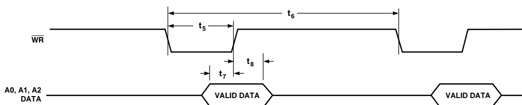
Figure 3. Parallel Timing
