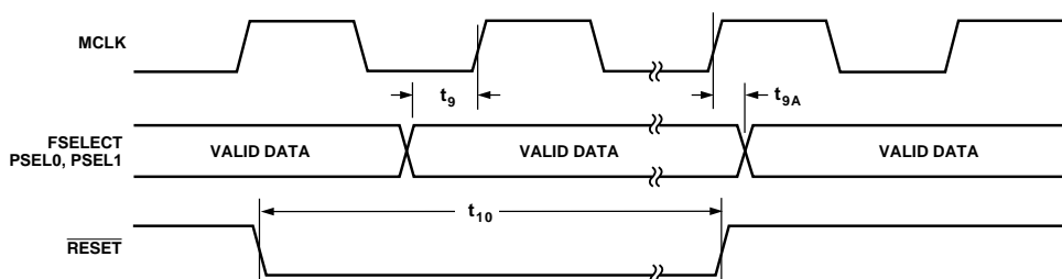
Figure 4. Control Timing
