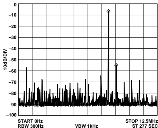
Figure 19. f_{MCLK} = 25 \text{ MHz} , f_{OUT} = 8.1 \text{ MHz} , Frequency Word = 52F1A9FC
