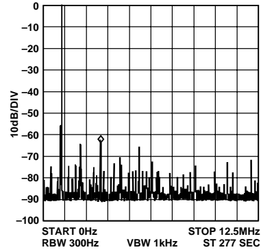
Figure 12. f_{MCLK} = 25 \text{ MHz} , f_{OUT} = 1.1 \text{ MHz} , Frequency Word = B439581
