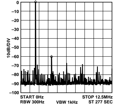
Figure 13. f_{MCLK} = 25 \text{ MHz} , f_{OUT} = 2.1 \text{ MHz} , Frequency Word = 15810625
