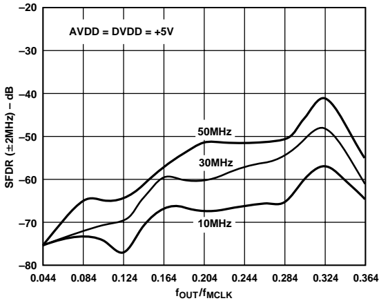
Figure 9. Wide Band SFDR vs. f_{OUT}/f_{MCLK} for Various MCLK Frequencies
