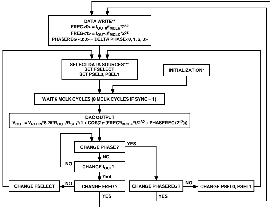
Figure 20. Flowchart for AD9835 Initialization and Operation
