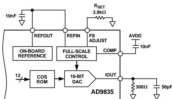
Figure 1. Test Circuit with Which Specifications Are Tested
