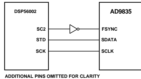
Figure 27. AD9835-to-DSP56002 Interface
