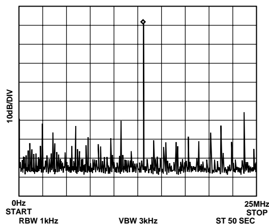
Figure 17. f_{MCLK} = 50 MHz, f_{OUT} = 13.1 MHz. Frequency Word = 43126E98
