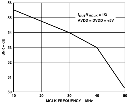
Figure 10. SNR vs. MCLK Frequency
