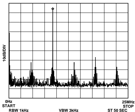
Figure 15. f_{MCLK} = 50 MHz, f_{OUT} = 9.1 MHz. Frequency Word = 2E978D50
