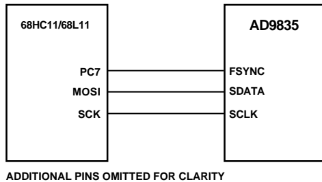
Figure 25. 68HC11/68L11-to-AD9835 Interface
