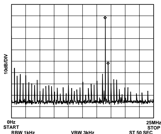
Figure 18. f_{MCLK} = 50 MHz, f_{OUT} = 16.5 MHz. Frequency Word = 547AE148
