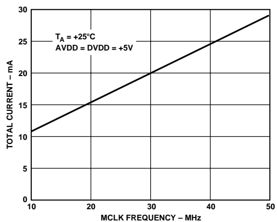
Figure 6. Typical Current Consumption vs. MCLK Frequency
