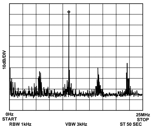
Figure 16. f_{MCLK} = 50 MHz, f_{OUT} = 11.1 MHz. Frequency Word = 38D4FDF4
