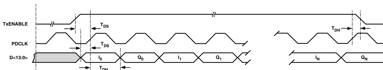
Figure 19. 14-Bit Parallel Port Timing Diagram—Quadrature Modulation Mode
