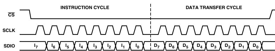
Figure 27. Serial Port Writing Timing—Clock Stall Low
