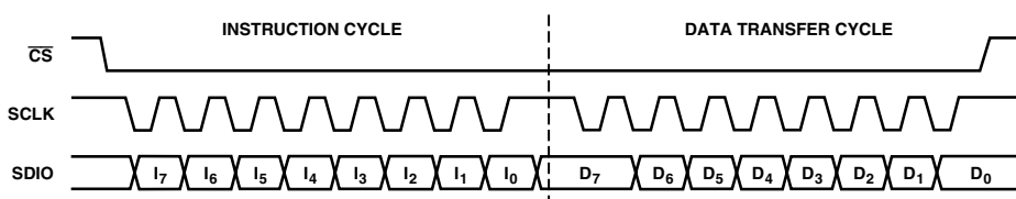
Figure 29. Serial Port Write Timing—Clock Stall High
