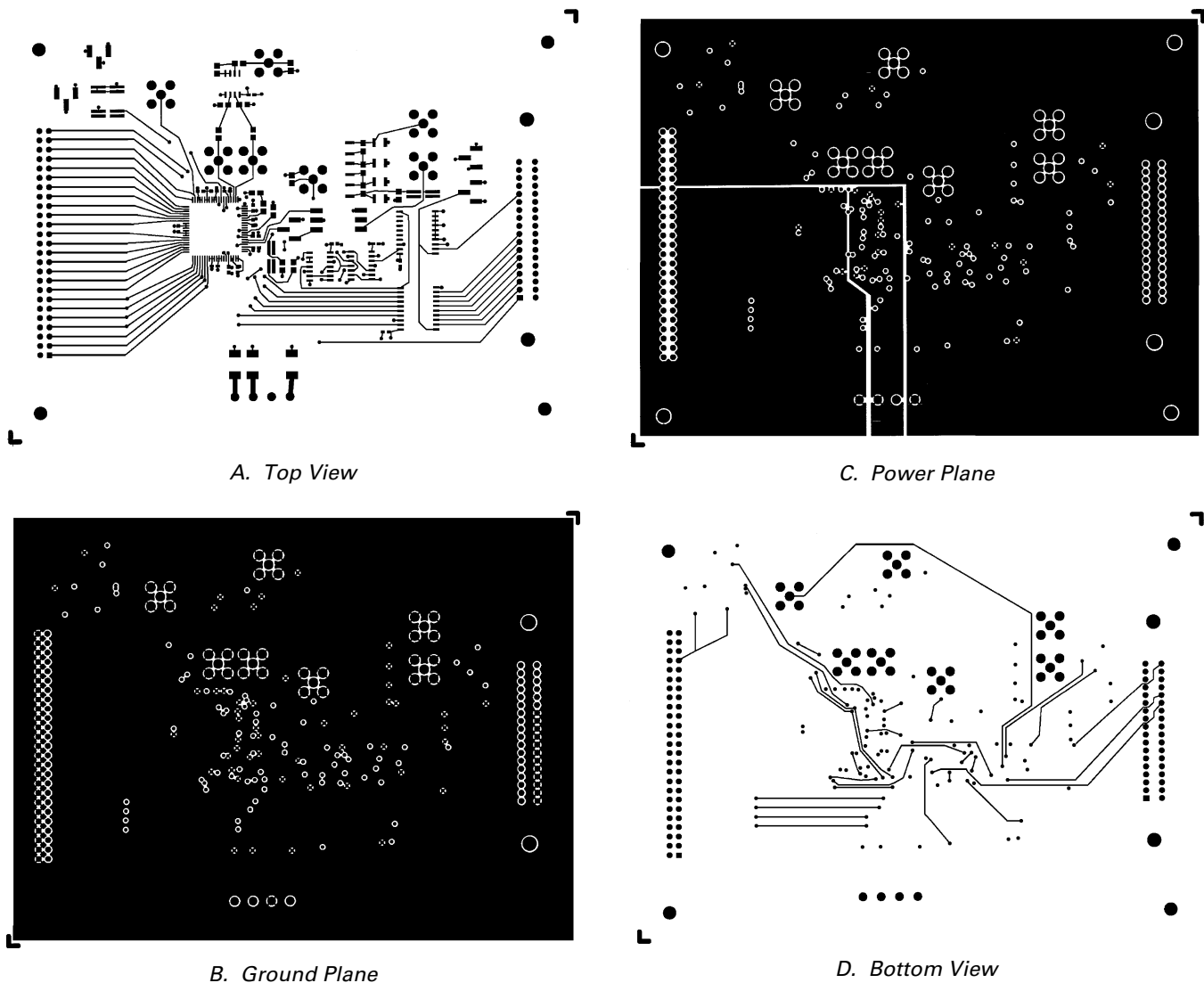
Figure 34. Application-Example Circuits
