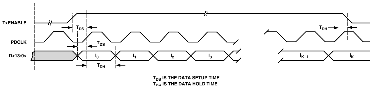
Figure 20. 14-Bit Parallel Port Timing Diagram—Interpolating DAC Mode
