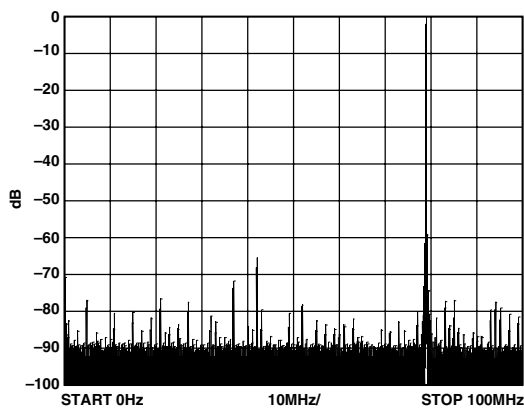
Figure 8. 79 MHz Single-Tone Output
