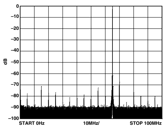
Figure 6. 65 MHz Single-Tone Output
