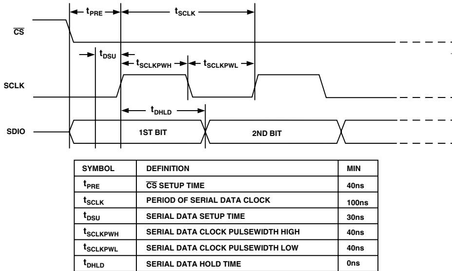
Figure 25. Timing Diagram for Data Write to AD9857
