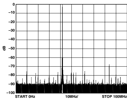
Figure 7. 42 MHz Single-Tone Output
