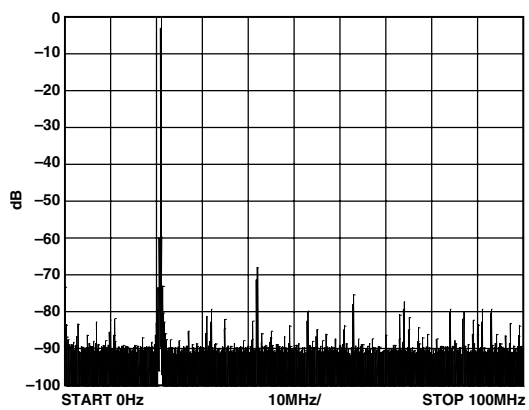
Figure 5. 21 MHz Single-Tone Output
