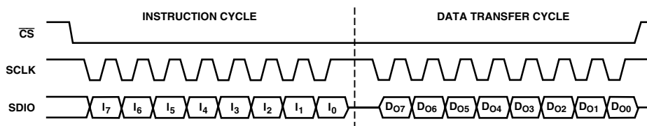
Figure 30. 2-Wire Serial Port Read Timing—Clock Stall High
