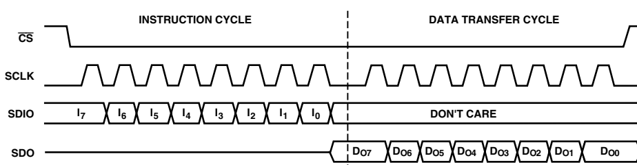
Figure 28. 3-Wire Serial Port Read Timing—Clock Stall Low
