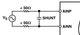
Figure 20. Simple ADC Drive Configuration
