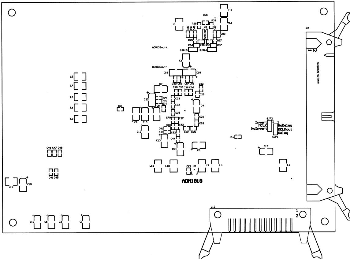
Figure 33. Evaluation Board PCB, Assembly Bottom Side
