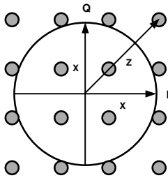
Figure 13. 16-Quadrature Modulation
