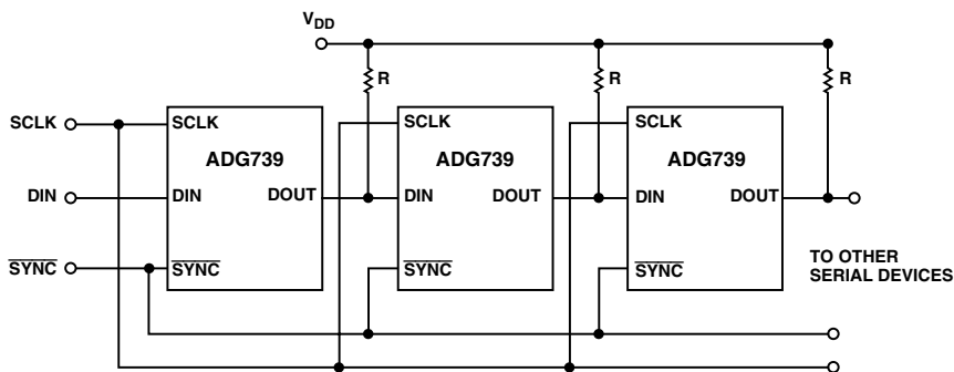
Figure 20. Multiple ADG739 Devices in a Daisy-Chained Configuration
