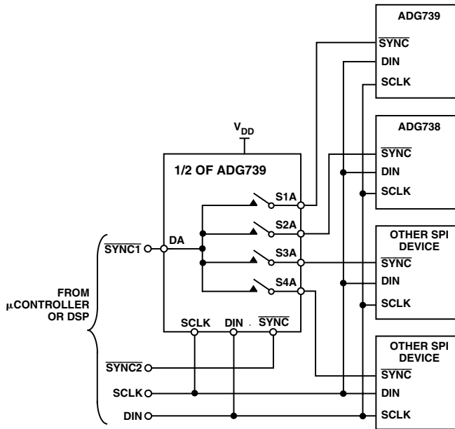
Figure 19. Addressing Multiple Serial Devices Using an ADG739
