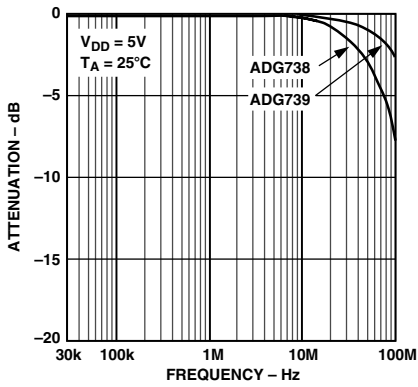
Figure 14. On Response vs. Frequency
