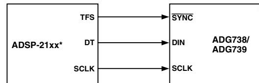
Figure 16. ADSP-21xx to ADG738/ADG739 Interface
