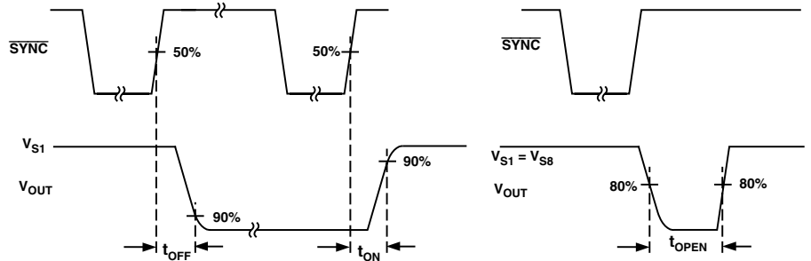
Test Circuit 5. Switching Times and Break-Before-Make Times
