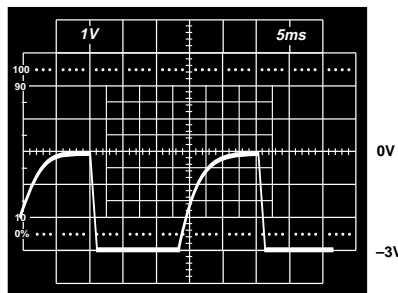
Figure 9. Start-Up Under Full Load
