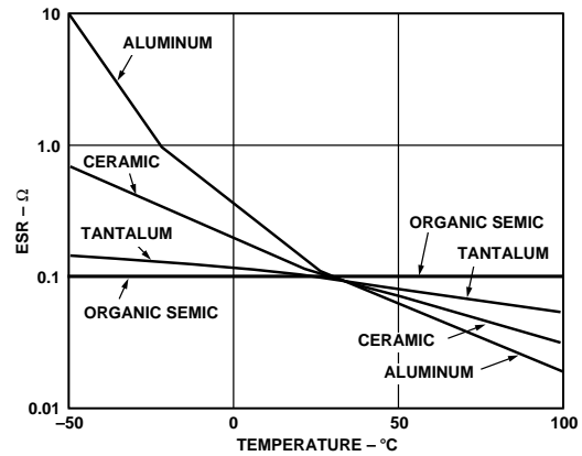
Figure 16. ESR vs. Temperature
