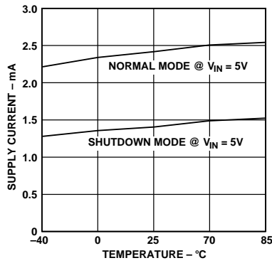
Figure 3. Supply Current vs. Temperature
