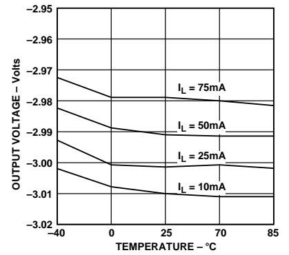
Figure 4. Output Voltage vs. Temperature
