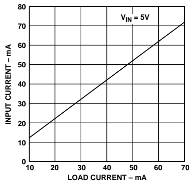
Figure 6. Average Input Current vs. Load Current
