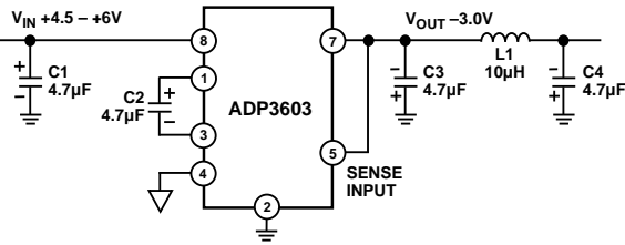
Figure 17. Circuit with Improved Output Ripple & Noise Voltage
