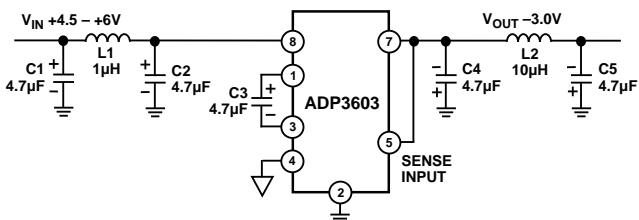
Figure 21. ADP3603 Evaluation Board Circuit Diagram
