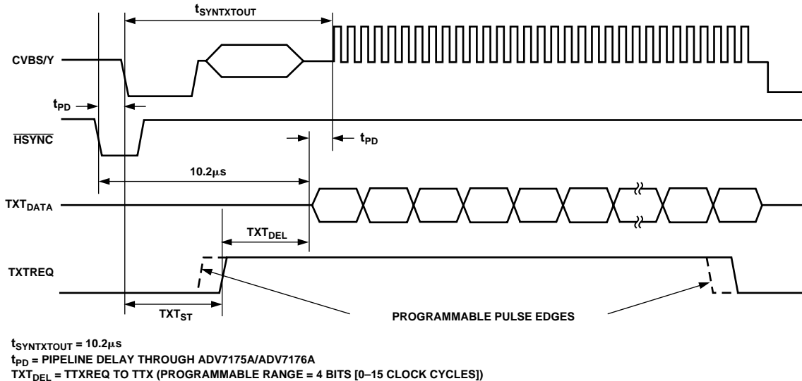
Figure 48. Teletext Functionality Diagram
