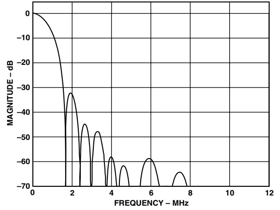
Figure 25. Chroma CIF Filter
