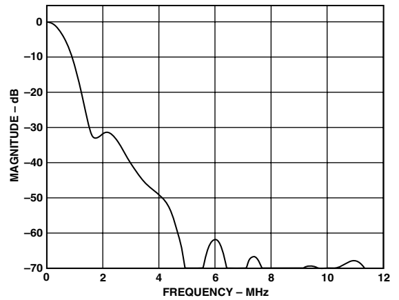
Figure 26. Chroma QCIF Filter
