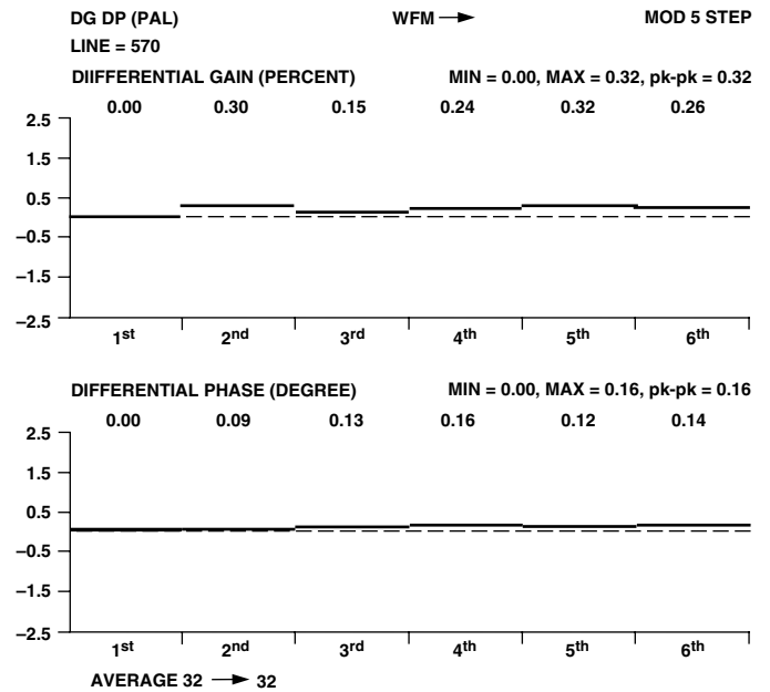
Figure 137. PAL DG DP Measurement
