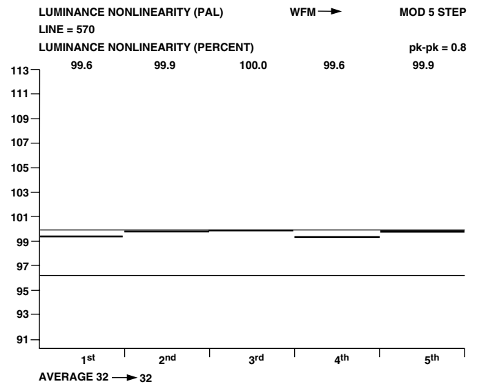
Figure 138. PAL Luminance Nonlinearity
