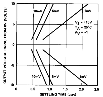
SETTLING TIME
