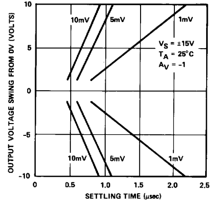
SETTLING TIME
