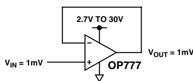
Figure 46. Follower Circuit
