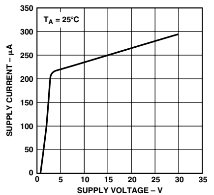
Figure 9. Supply Current vs. Supply Voltage
