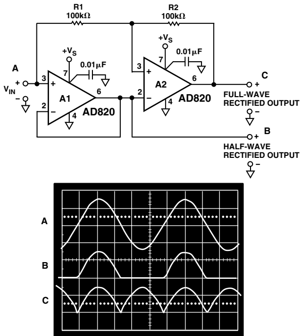
Figure 20. Single Supply Half- and Full-Wave Rectifier
