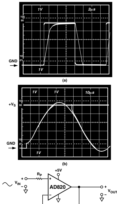
Figure 14. (a) Response with R_P = 0 ; V_{IN} from 0 to +V_S (b) V_{IN} = 0 to +V_S + 200 mV V_{OUT} = 0 to +V_S R_P = 49.9 k \Omega
