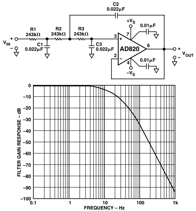
Figure 22. 10 Hz Sallen Key Low-Pass Filter
