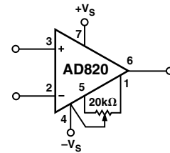
Figure 19. Offset Null
