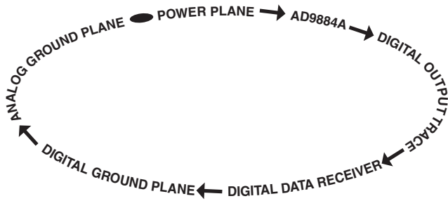
Figure 27. Current Loop
