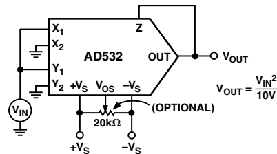
Figure 12. Squarer Connection
