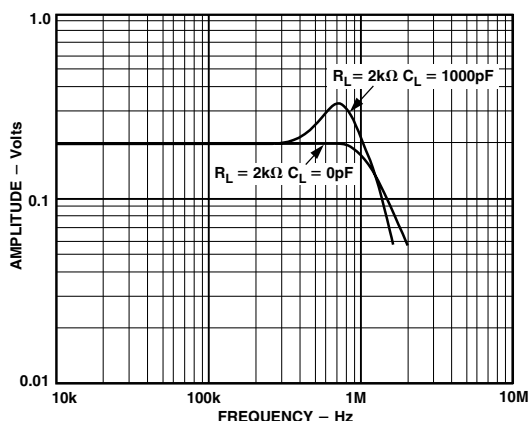
Figure 7. Frequency Response, Multiplying
