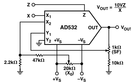
Figure 13. Divider Connection
