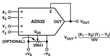
Figure 11. Multiplier Connection
