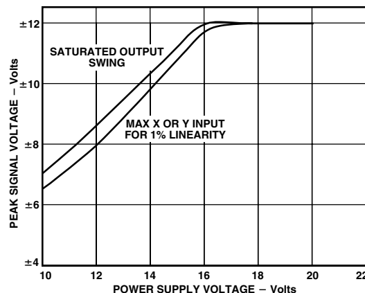
Figure 9. Signal Swing vs. Supply
