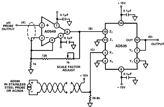
Figure 46. Temperature Compensated pH Probe Amplifier
