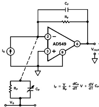
Figure 26. Sources of Parasitic Leakage Currents
