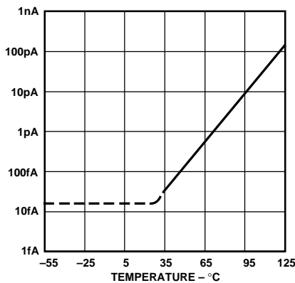
Figure 24. AD549 Input Bias Current vs. Ambient Temperature
