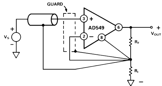
Figure 29. Noninverting Amplifier with Guard
