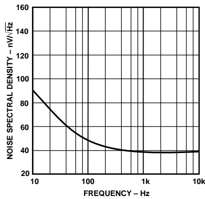
Figure 11. Input Voltage Noise Spectral Density
