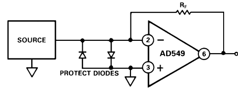
Figure 39. Input Voltage Clamp with Diodes
