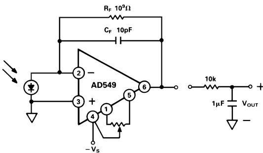
Figure 41. Photodiode Preamp
