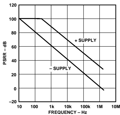
Figure 16. PSRR vs. Frequency
