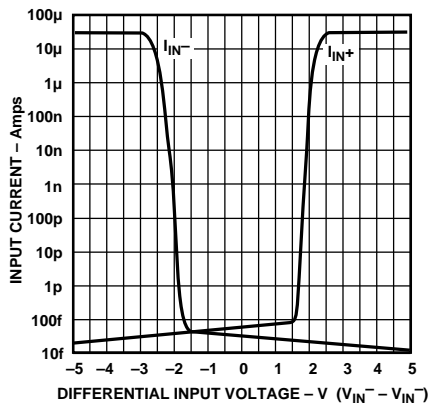
Figure 36. Input Current vs. Differential Input Voltage
