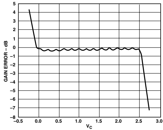
Figure 6. Gain Error for Cascaded Stages—Sequential Control
