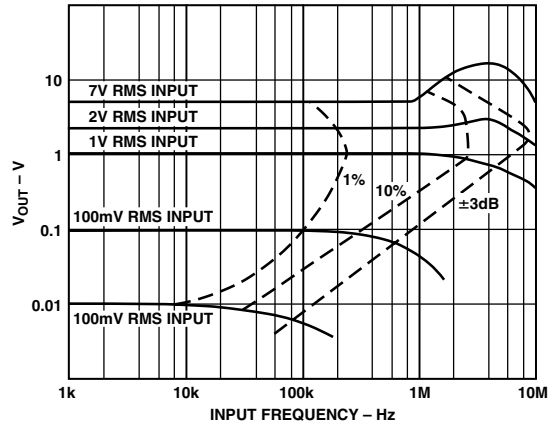
Figure 10. Frequency Response
