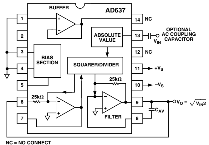
Figure 2. Standard RMS Connection
