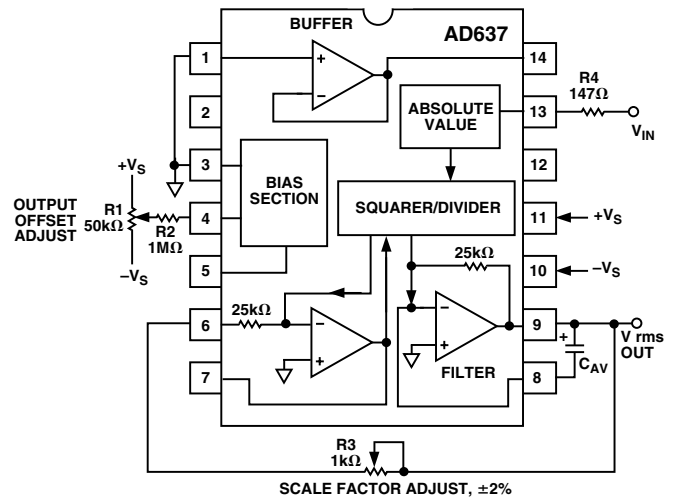
Figure 5. Optional External Gain and Offset Trims
