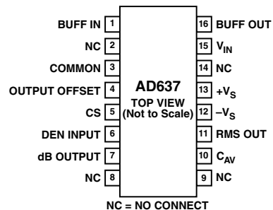
16-Lead SOIC
