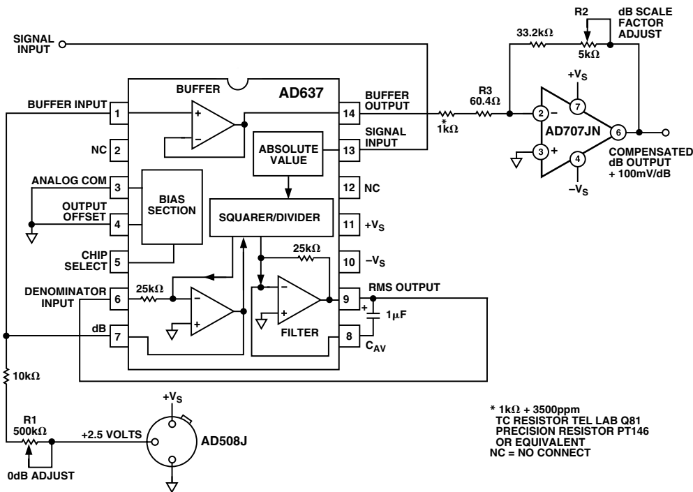
Figure 14. dB Connection
