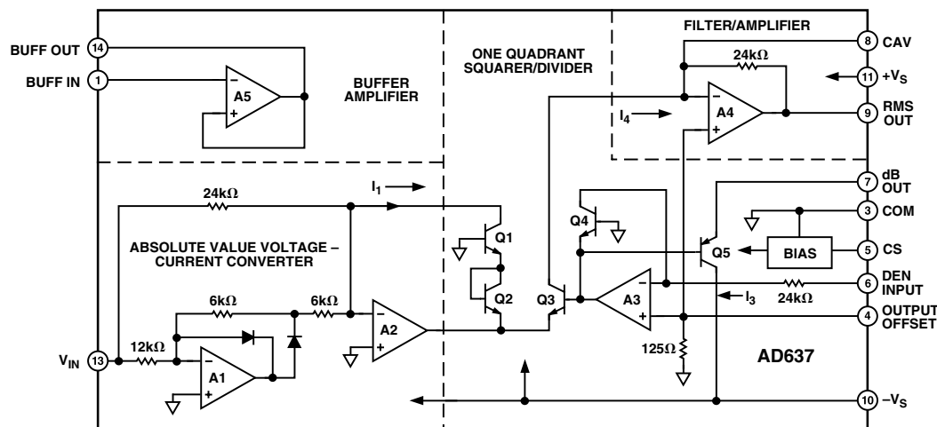
Figure 1. Simplified Schematic
