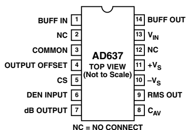
14-Lead DIP
