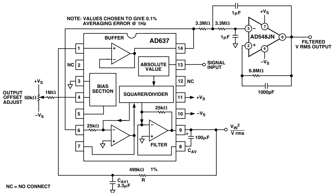
Figure 15. AD637 as a Low Frequency RMS Converter
