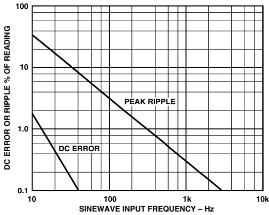
Figure 7. Comparison of Percent DC Error to the Percent Peak Ripple over Frequency Using the AD637 in the Standard RMS Connection with a 1 \times \mu F C_{AV}
