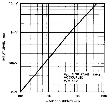
Figure 9. -3 dB Frequency vs. RMS Input Level (Pin 2)
