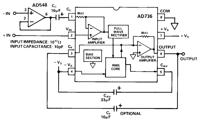
Figure 20. Differential Input Connection
