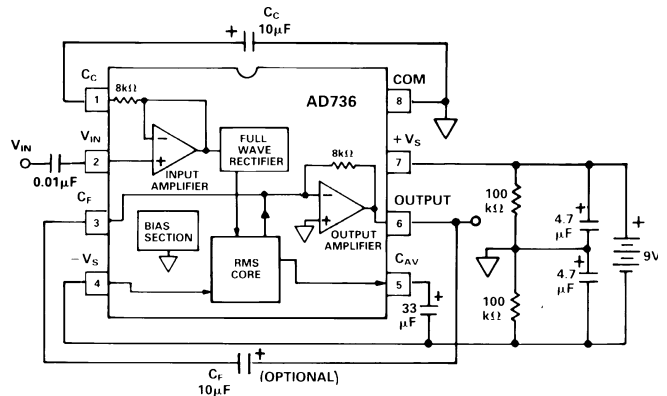
Figure 22. Battery Powered Option
