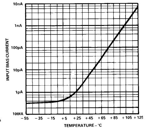
Figure 15. Pin 2 Input Bias Current vs. Temperature
