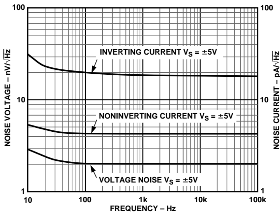
Figure 29. Noise vs. Frequency
