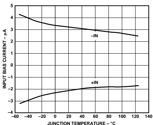
Figure 24. Input Bias Current vs. Temperature
