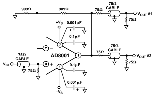
Figure 47. Video Line Driver
