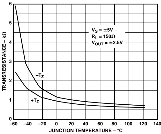
Figure 28. Transresistance vs. Temperature
