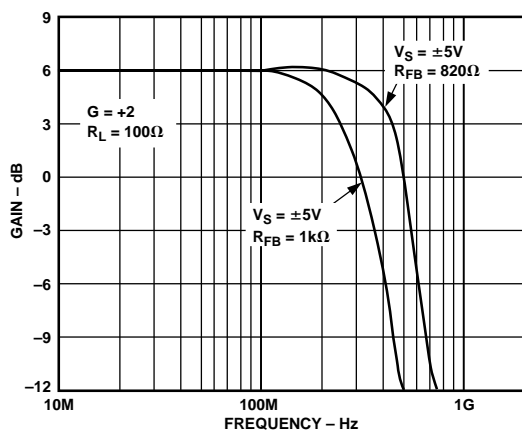
Figure 1. Frequency Response of AD8001
