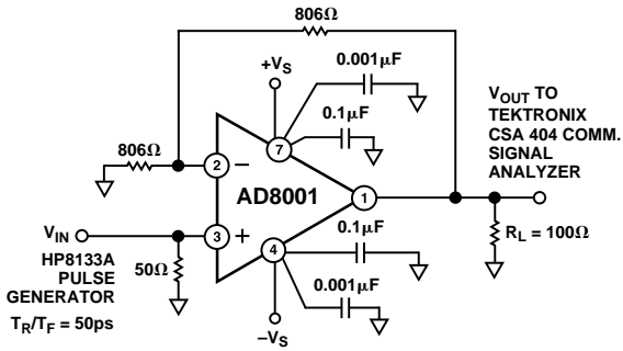
Figure 4. Test Circuit, Gain = +2
