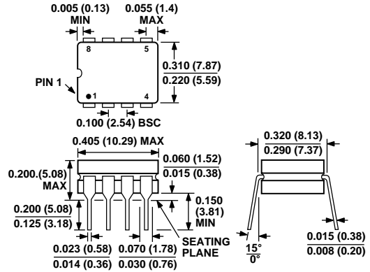
8-Lead Cerdip (Q-8)
