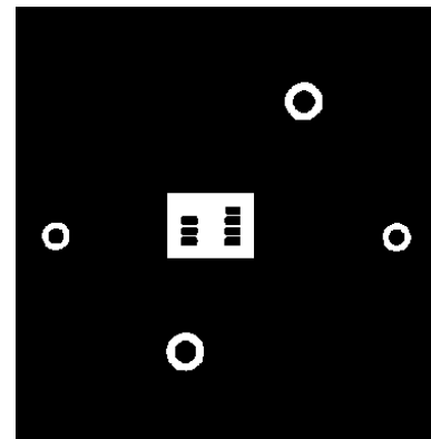
Figure 52. Evaluation Board Layout (Component Side)
