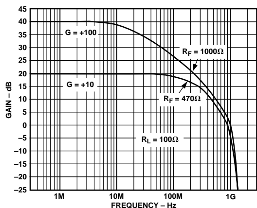
Figure 22. Frequency Response, G = +10 , G = +100
