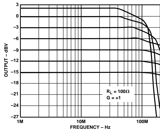
Figure 21. Large Signal Frequency Response, G = +1
