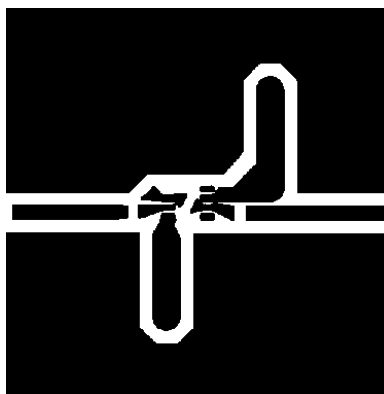
Figure 51. Evaluation Board Layout (Solder Side)
