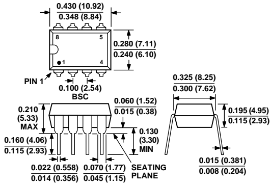
8-Lead Plastic DIP (N-8)
