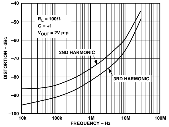
Figure 20. Distortion vs. Frequency, R_L = 100\ \Omega
