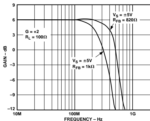
Figure 10. Frequency Response, G = +2
