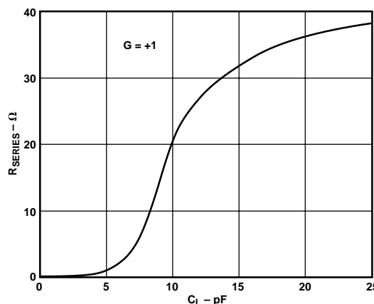
Figure 45. Recommended R_{SERIES} vs. Capacitive Load
