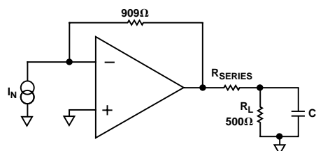
Figure 44. Driving Capacitive Loads
