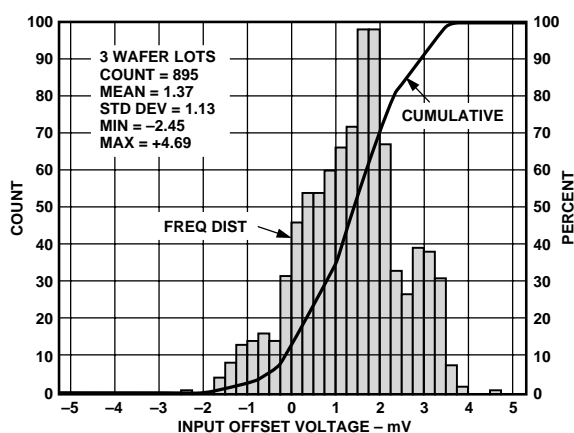
Figure 39. Input Offset Voltage Distribution
