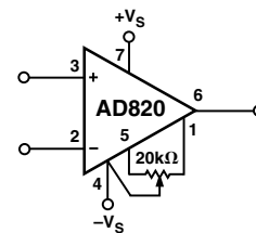
Figure 19. Offset Null
