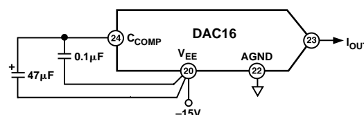
Figure 21a. Recommended Compensation Scheme to V_{\text{EE}}
