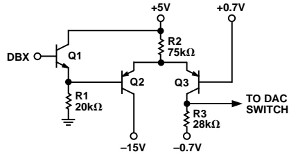
Figure 5. Equivalent Circuit of a DAC16 Digital Input
