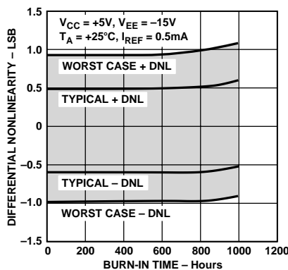
Figure 16. Differential Nonlinearity vs. Time Accelerated by Burn-In
