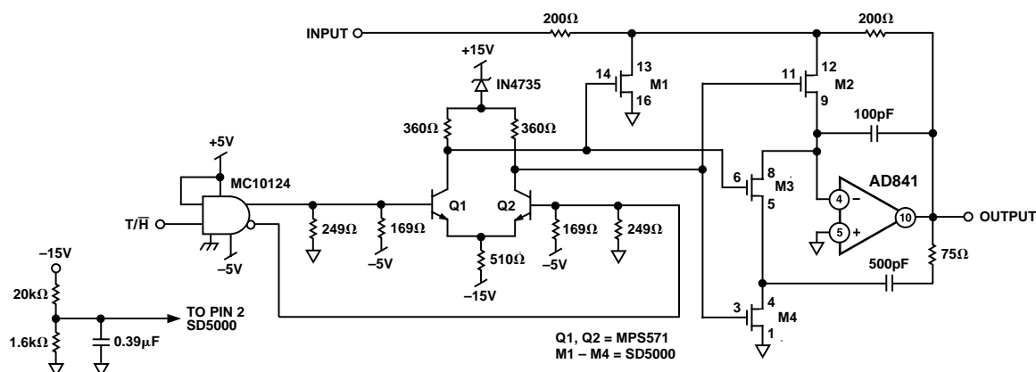
Figure 27. A High Performance Deglitching Circuit
