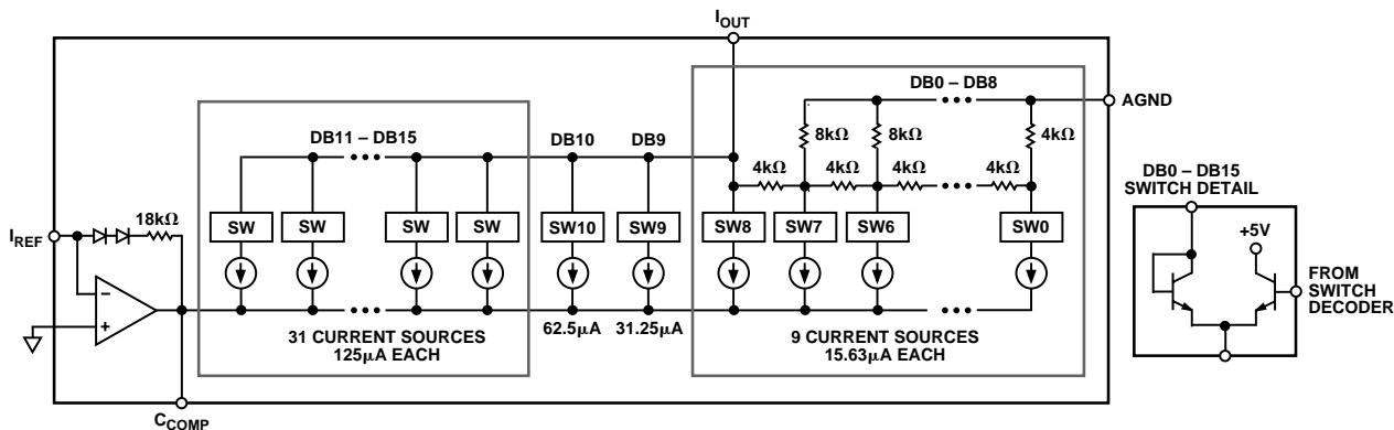
Figure 3. DAC16 Architecture
