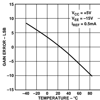
Figure 10. Gain Error vs. Temperature
