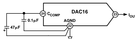
Figure 21b. Recommended Compensation Scheme to AGND
