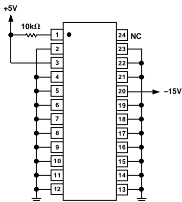
Figure 2. Burn-In Diagram
