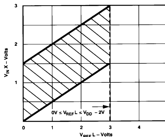
Figure 20. DAC-8841 Input Voltage Operating Boundaries
