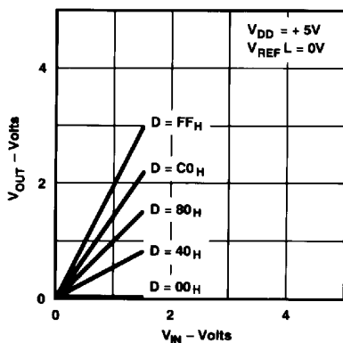
DAC8841 INPUT-OUTPUT VOLTAGE RANGE
