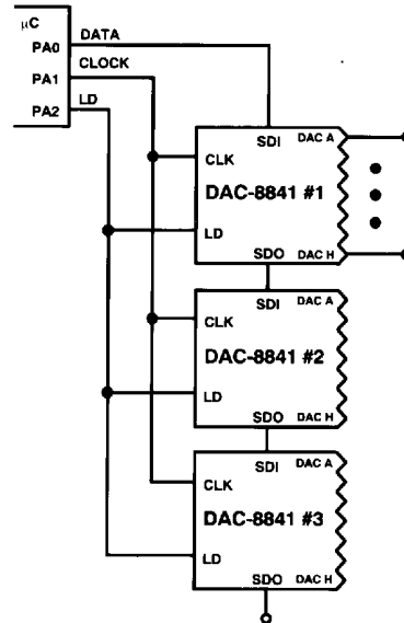
Figure 21. Three-Wire Interface
