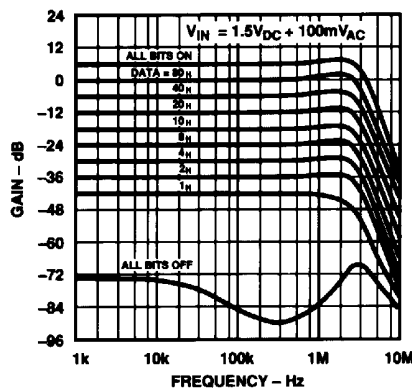
Figure 22. Gain ( V_{OUT}/V_{IN} ) and Feedthrough vs. Frequency
