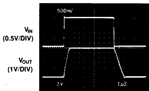
Figure 11. Pulse Response
