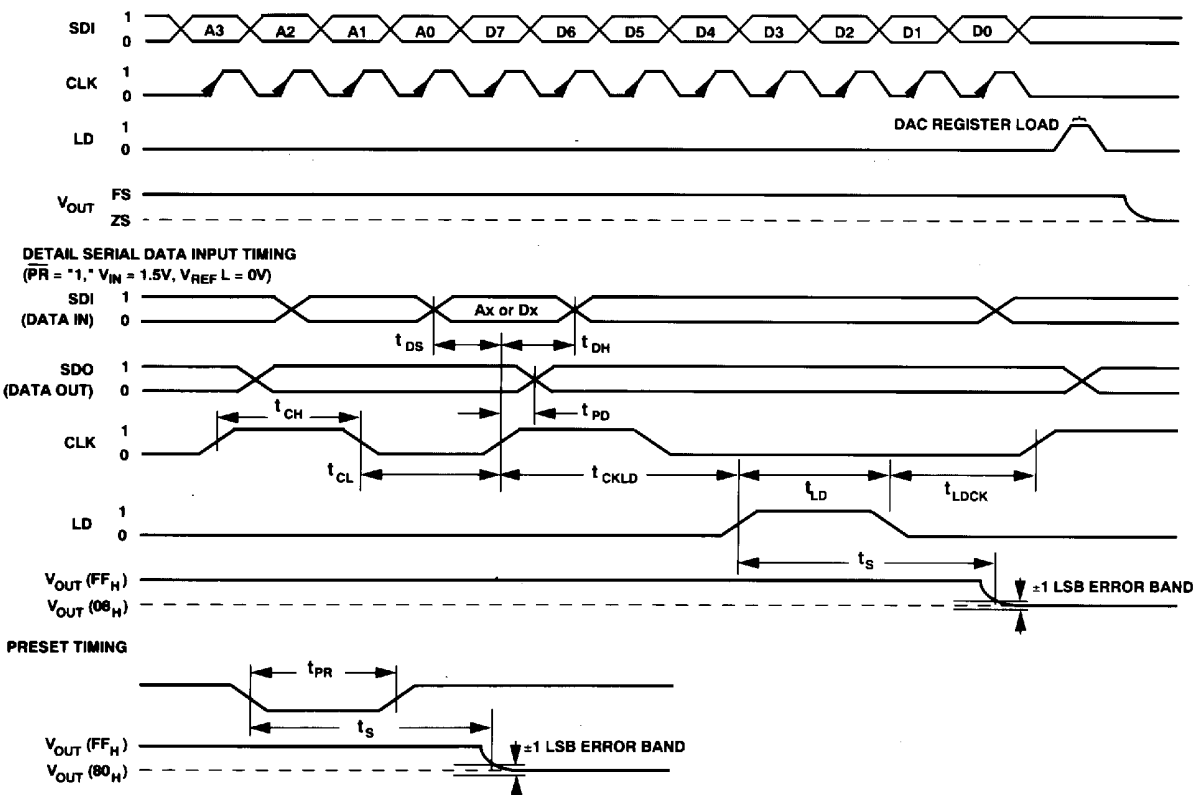
Figure 1. Timing Diagram
