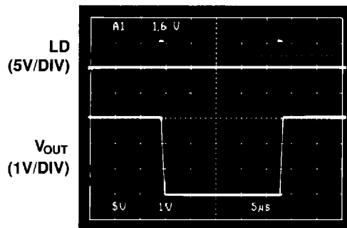
Figure 12. Settling Time
