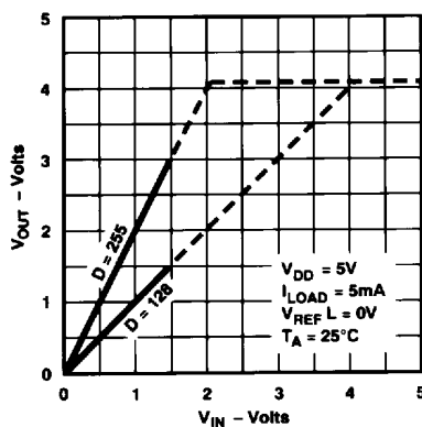
Figure 8. Full-Scale Output to Positive Saturation
