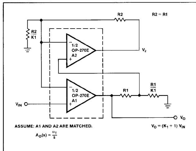
FIGURE 10: Low Phase Error Amplifier
