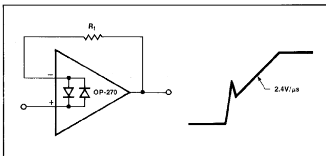
FIGURE 9: Pulsed Operation
