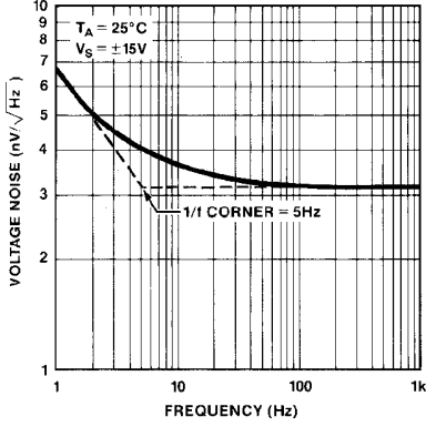
VOLTAGE NOISE DENSITY vs FREQUENCY
