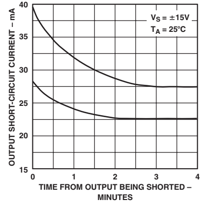
TPC 18. Output Short-Circuit Current vs. Time
