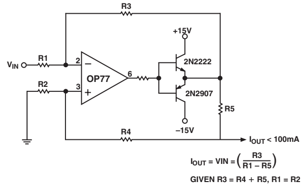
Figure 10. 100 mA Current Source
