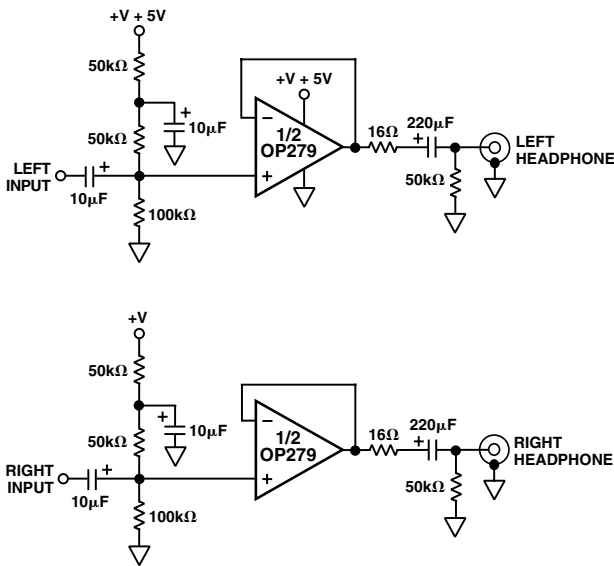
Figure 13. A Single-Supply, Stereo Headphone Driver
