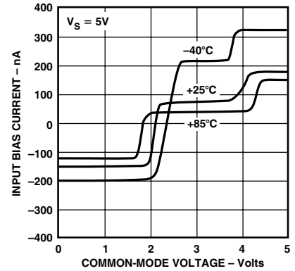
TPC 3. Input Bias Current vs. Common-Mode Voltage
