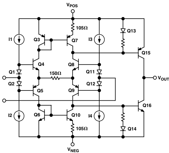
Figure 2. OP179/OP279 Equivalent Output Circuit
