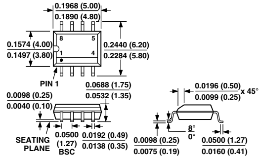
8-Lead Narrow-Body SO (SO-8)
