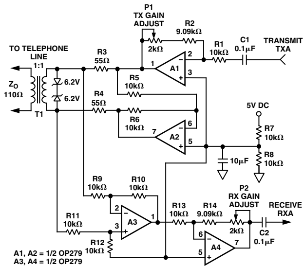
Figure 10. A Single-Supply Direct Access Arrangement for Modems
