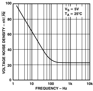
TPC 19. Voltage Noise Density vs. Frequency
