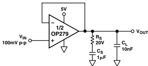
Figure 5. Snubber Network Compensates for Capacitive Load
