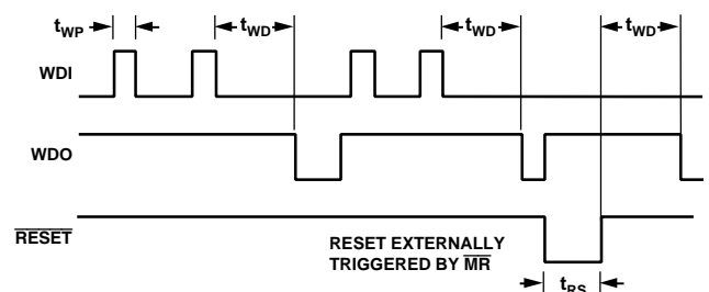
Figure 4. Watchdog Timing
