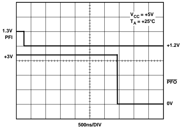
Figure 10. PFI Assertion Response Time
