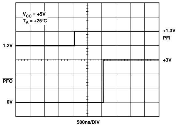
Figure 11. PFI Deassertion Response Time
