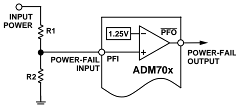
Figure 5. Power-Fail Comparator
