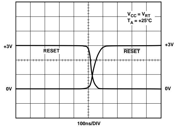
Figure 13. \overline{\text{RESET}} , RESET Deassertion
