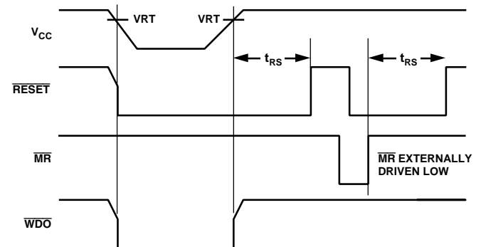
Figure 3. \overline{\text{RESET}} , \overline{\text{MR}} and \overline{\text{WDO}} Timing
