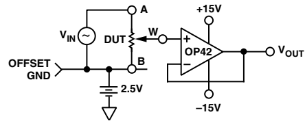
Test Circuit 7. Gain vs. Frequency
