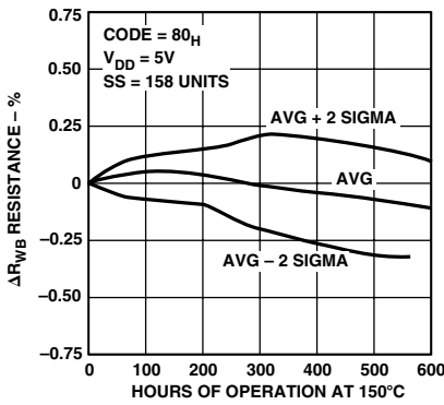
TPC 13. Long-Term Drift Accelerated by Burn-In
