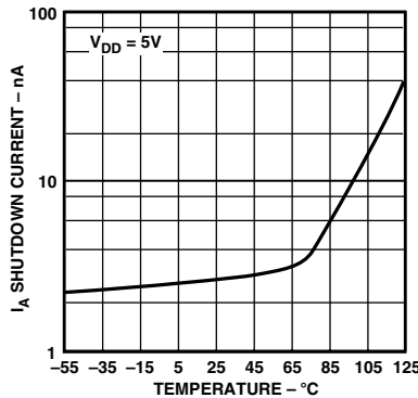
TPC 26. Shutdown Current vs. Temperature
