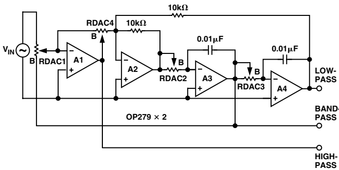
Figure 10. Programmable State Variable Active Filter
