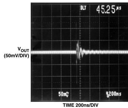
TPC 17. Digital Feedthrough vs. Time
