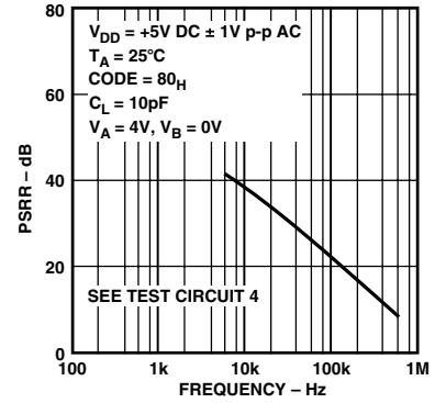
TPC 21. Power Supply Rejection vs. Frequency
