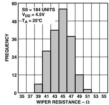
TPC 6. 50 kΩ Wiper-Contact-Resistance Histogram
