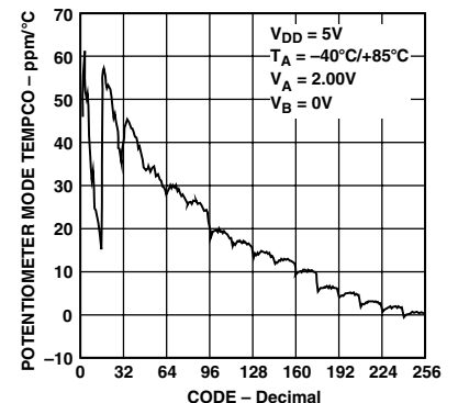
TPC 9. DV_{WB}/DT Potentiometer Mode Tempco
