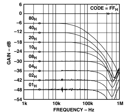
TPC 18. 100 k \Omega Gain vs. Frequency vs. Code
