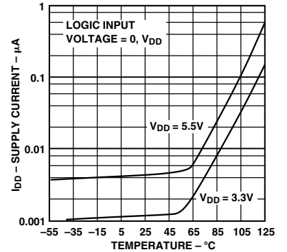
TPC 27. Supply Current vs. Temperature
