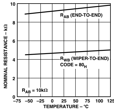
TPC 8. Nominal Resistance vs. Temperature
