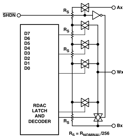
Figure 3. AD8402/AD8403 Equivalent VR (RDAC) Circuit
