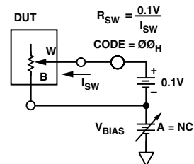
Test Circuit 8. Incremental ON Resistance
