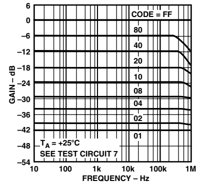
TPC 12. 10 k \Omega Gain vs. Frequency
