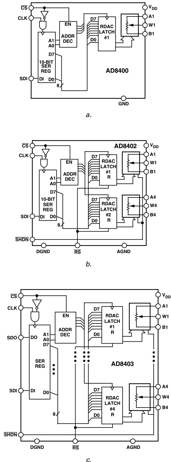
Figure 4. Block Diagrams
