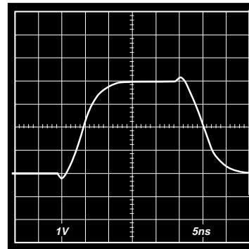
Figure 6. Inverting Configuration, G = -1
