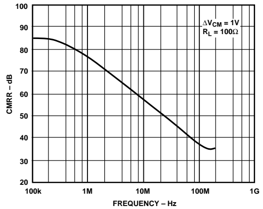
Figure 42. AD8048 CMRR vs. Frequency
