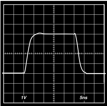
Figure 9. Noninverting Configuration, G = +2
