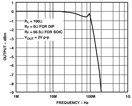
Figure 18. AD8047 Large Signal Frequency Response, G = +1
