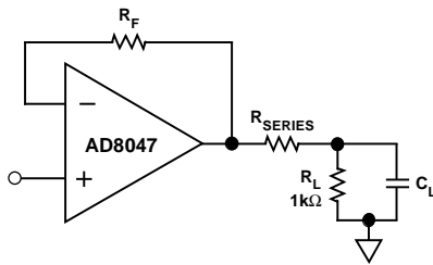
Figure 54. Driving Capacitive Loads
