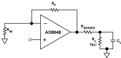
Figure 56. Driving Capacitive Loads
