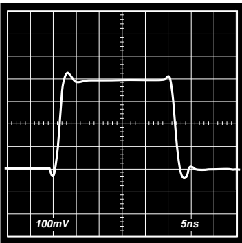
Figure 14. Small Signal Transient Response; V_O = 400\text{ mV p-p} , G = -1 , R_F = R_{IN} = 200\ \Omega
