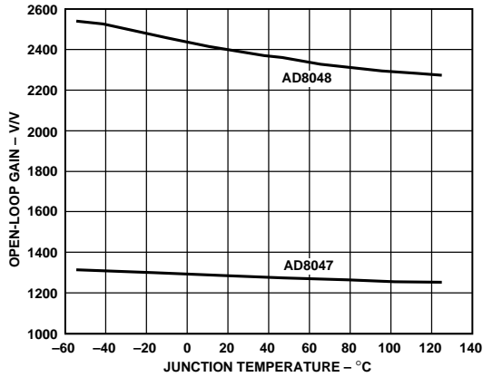
Figure 46. AD8047/AD8048 Open-Loop Gain vs. Temperature
