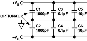
Supply Bypassing
