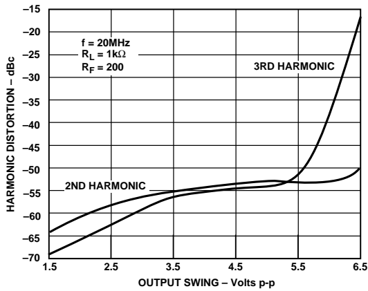
Figure 34. AD8048 Harmonic Distortion vs. Output Swing, G = +2
