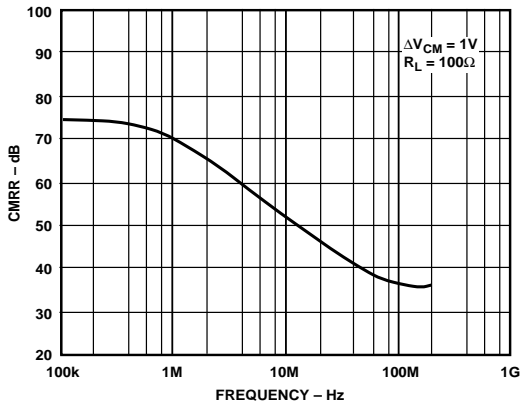
Figure 39. AD8047 CMRR vs. Frequency
