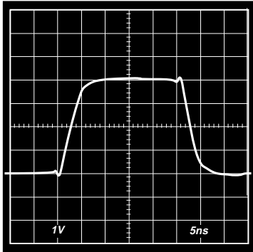
Figure 3. Noninverting Configuration, G = +1
