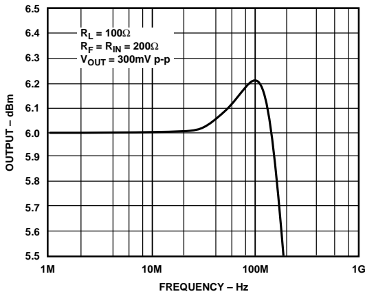
Figure 28. AD8048 0.1 dB Flatness, G = +2
