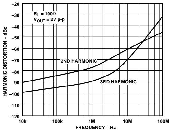
Figure 33. AD8048 Harmonic Distortion vs. Frequency, G = +2
