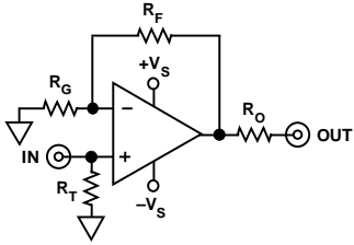
Noninverting Configuration
