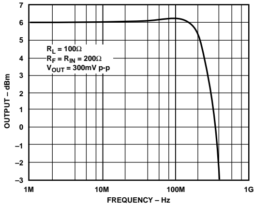
Figure 27. AD8048 Small Signal Frequency Response, G = +2
