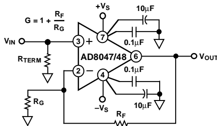
Figure 51. Noninverting Operation
