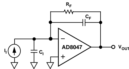
Figure 53. Transimpedance Configuration
