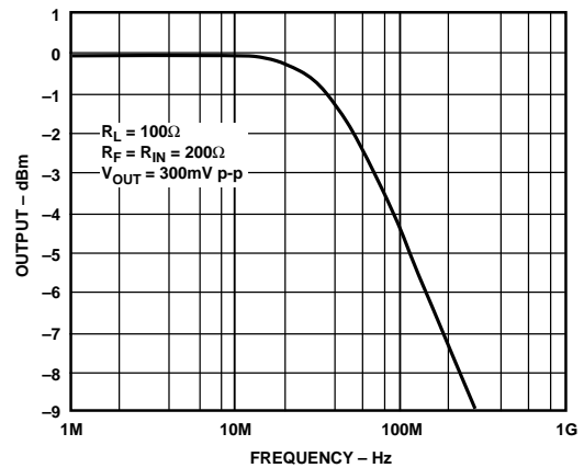
Figure 19. AD8047 Small Signal Frequency Response, G = -1
