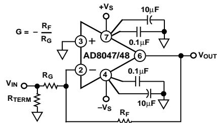
Figure 52. Inverting Operation
