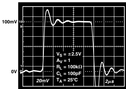
TPC 32. Small Signal Transient Response
