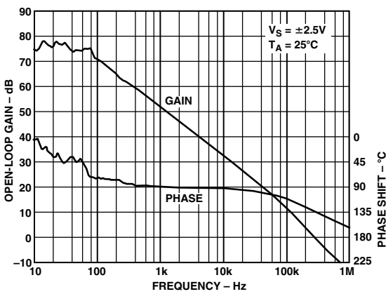
TPC 15. Open-Loop Gain and Phase vs. Frequency (No Load)
