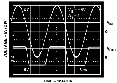
Figure 2. Output Voltage Phase Reversal Behavior
