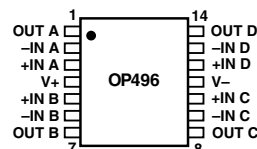
14-Lead TSSOP (RU Suffix)
