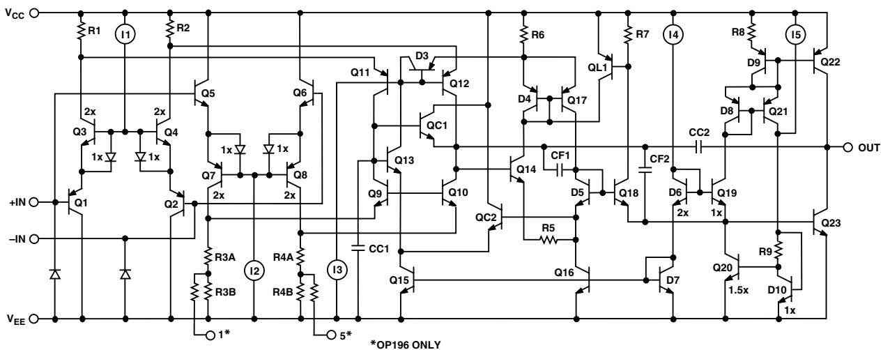
TPC 36. Simplified Schematic
