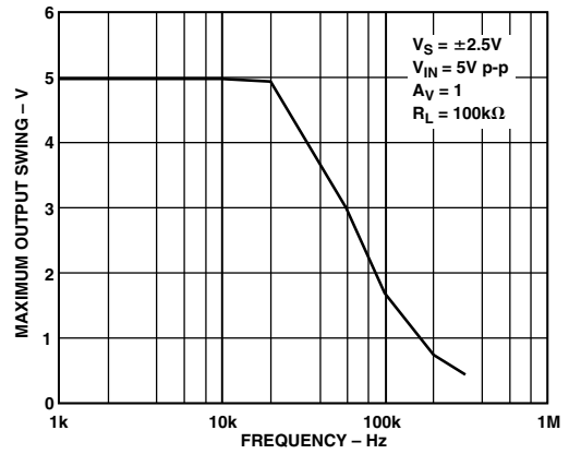
TPC 24. Maximum Output Swing vs. Frequency
