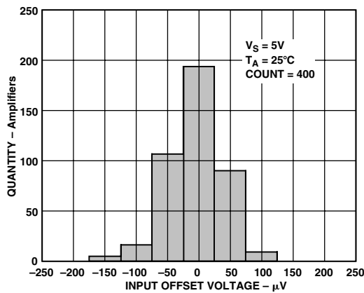
TPC 2. Input Offset Voltage Distribution
