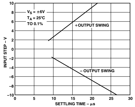
TPC 29. Settling Time to 0.1% vs. Step Size
