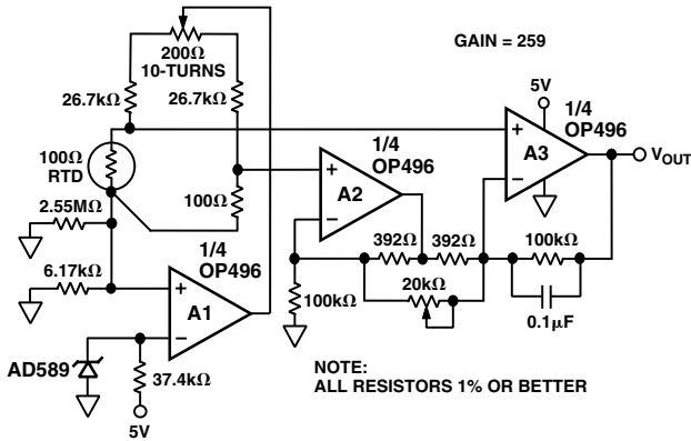
Figure 12. A Single-Supply RTD Amplifier
