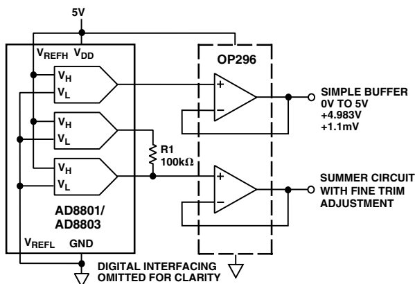
Figure 10. Buffering a TrimDAC Output TPC
