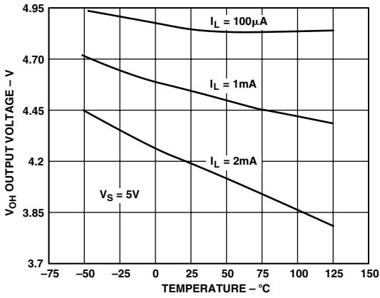
TPC 13. Output Voltage Swing vs. Temperature
