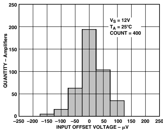
TPC 3. Input Offset Voltage Distribution
