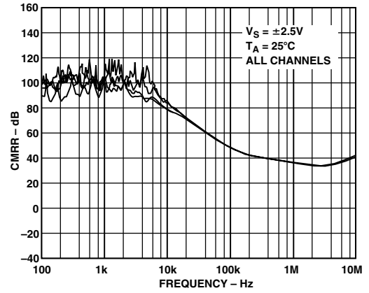
TPC 22. CMRR vs. Frequency
