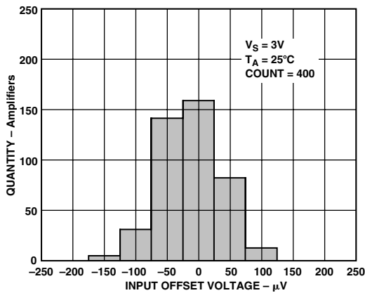
TPC 1. Input Offset Voltage Distribution
