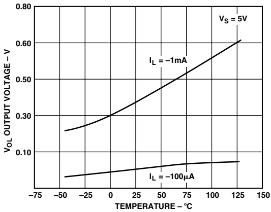
TPC 14. Output Voltage Swing vs. Temperature
