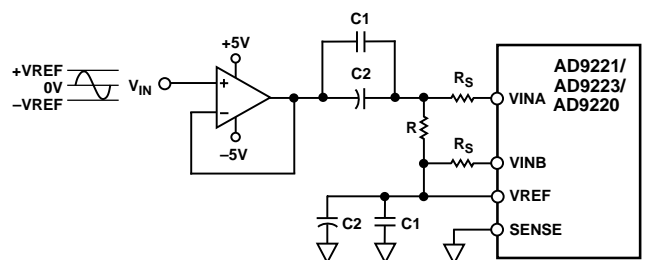
Figure 41. AC-Coupled Input
