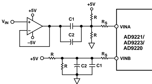
Figure 42. AC-Coupled Input-Flexible Input Span, V CM = 2 V
