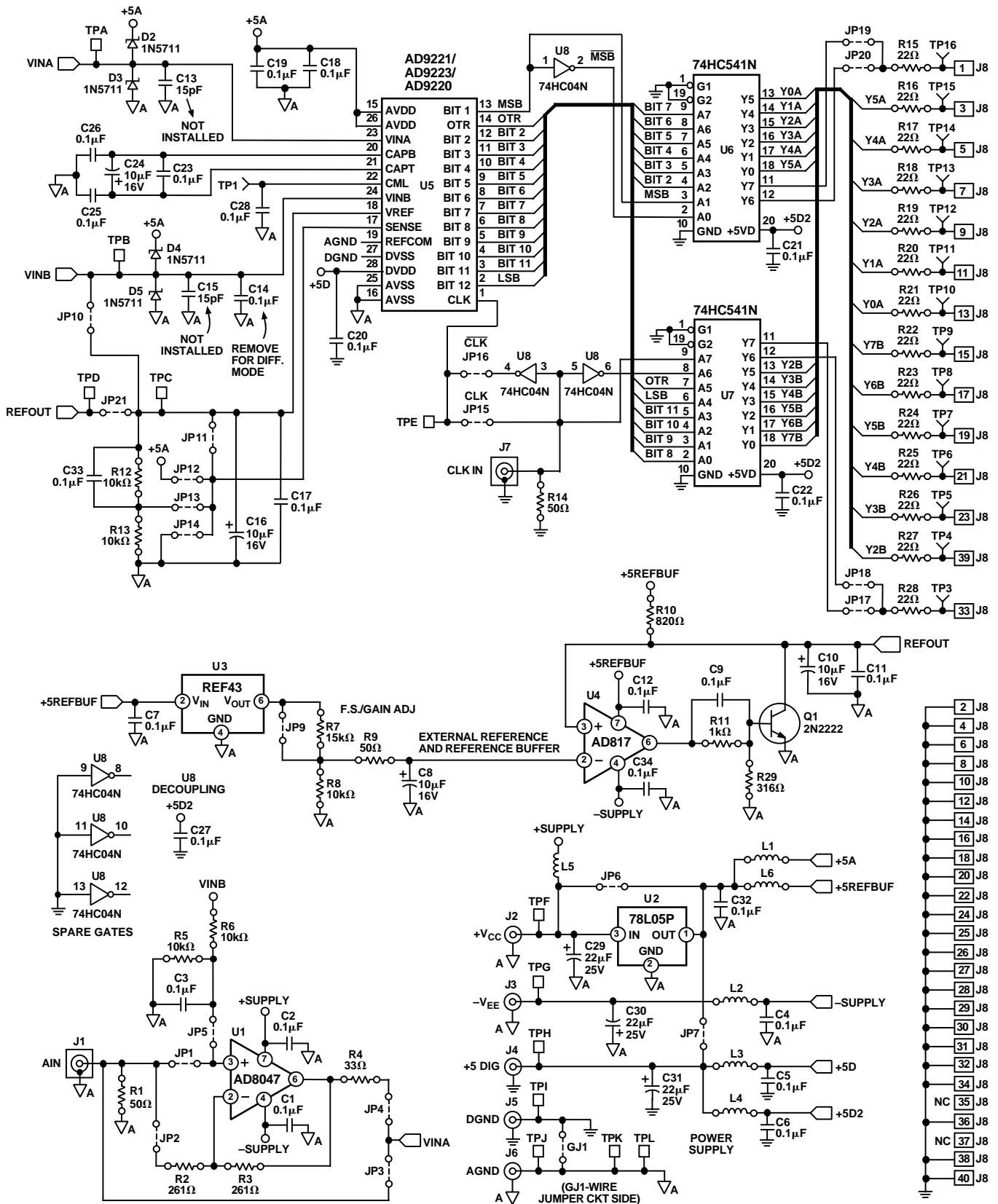
Figure 62. Evaluation Board Schematic
