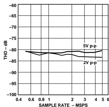
Figure 18. THD vs. Sample Rate ( A_{IN} = -0.5\text{ dB} , f_{IN} = 500\text{ kHz} , V_{CM} = 2.5\text{ V} )
