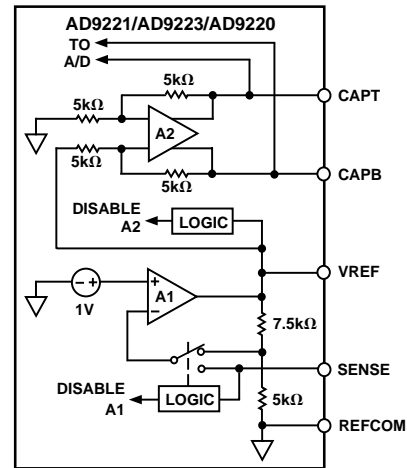
Figure 35. Equivalent Reference Circuit
