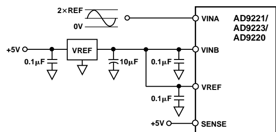
Figure 51. Input Range = 0 V to 2 \times \text{VREF}
