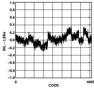
Figure 3. Typical INL
