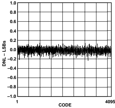
Figure 20. Typical DNL
