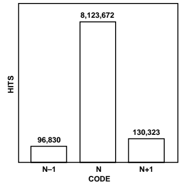
Figure 13. "Grounded-Input" Histogram (Input Span = 2 V p-p)
