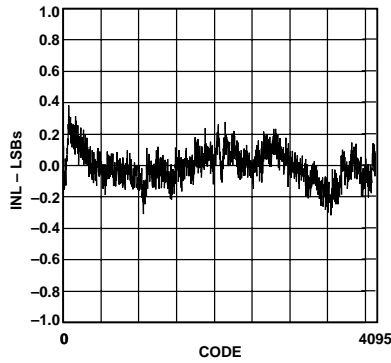
Figure 12. Typical INL
