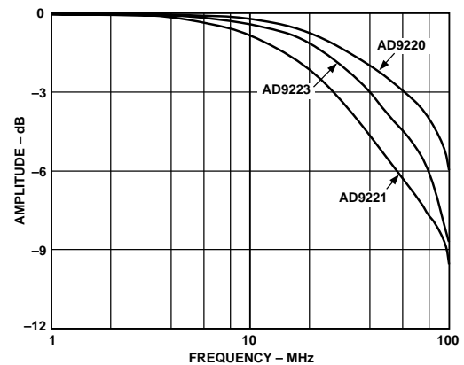
Figure 29. Full-Power Bandwidth
