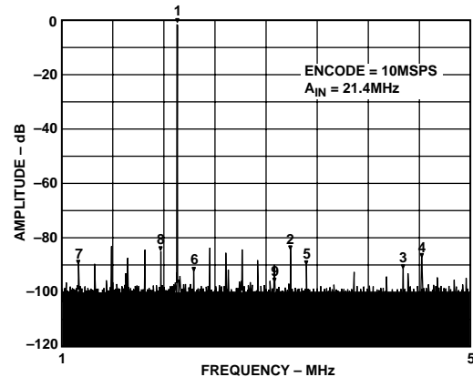
Figure 59. IF Sampling a 21.4 MHz Input Using the AD9220 ( V_{CM} = 2.5 \text{ V} , Input Span = 2 V p-p)
