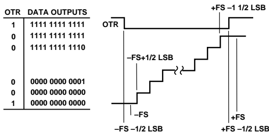
Figure 53. Output Data Format
