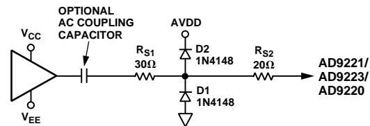
Figure 38. Simple Clamping Circuit
