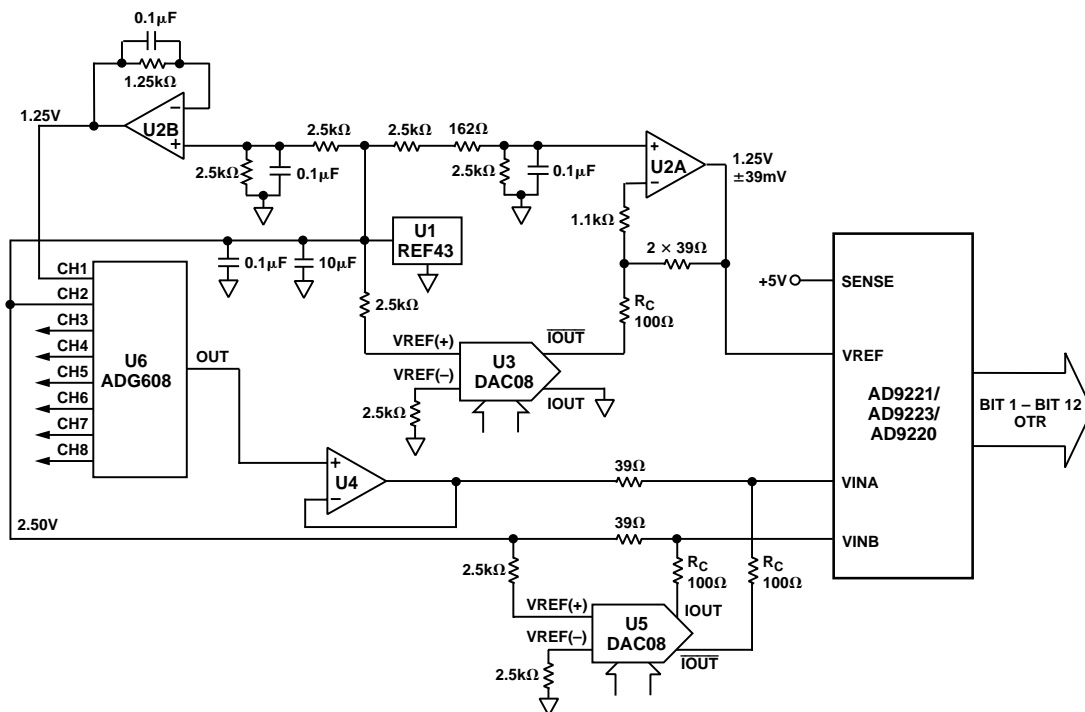
Figure 61. Typical Multichannel Data Acquisition System
