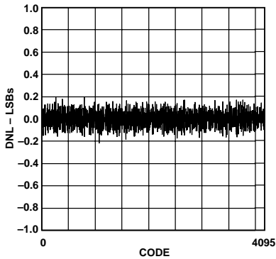
Figure 11. Typical DNL
