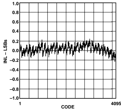
Figure 21. Typical INL
