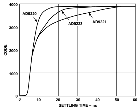
Figure 30. Settling Time
