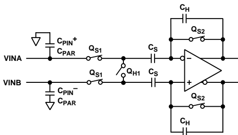
Figure 32. AD9221/AD9223/AD9220 Simplified Input Circuit
