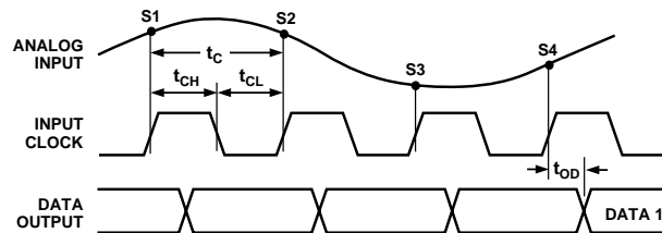
Figure 1. Timing Diagram
