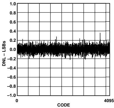
Figure 2. Typical DNL
