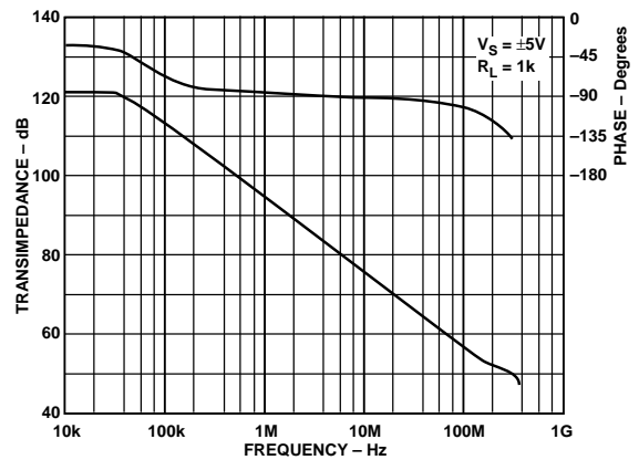
Figure 14. Open-Loop Transimpedance vs. Frequency (Relative to 1 Ω)
