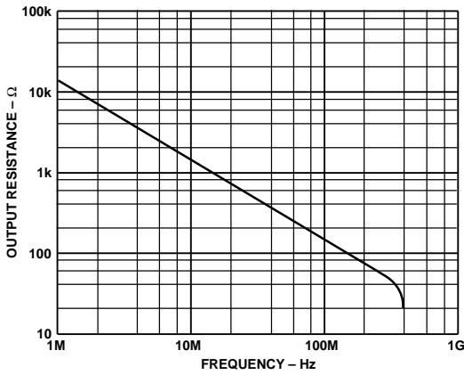
Figure 10. Output Resistance vs. Frequency, Disabled State
