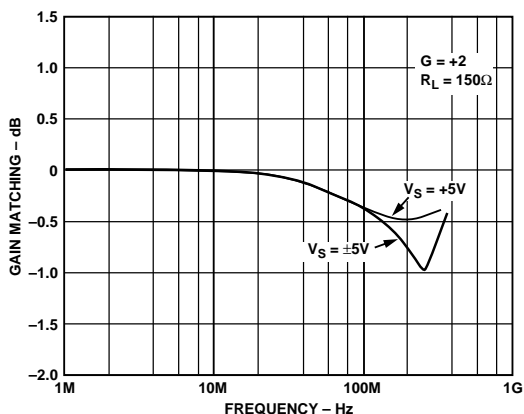
Figure 34. Closed-Loop Gain Matching vs. Frequency
