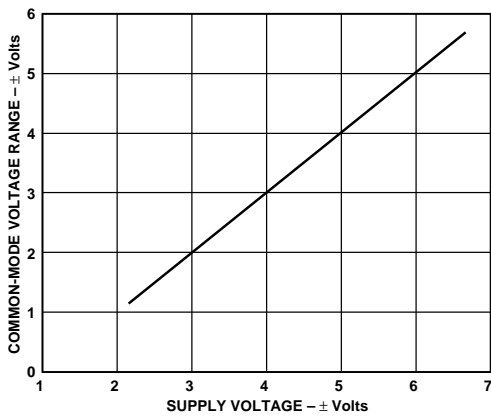
Figure 1. Input Common-Mode Voltage Range vs. Supply Voltage
