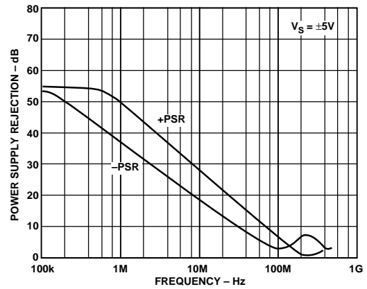
Figure 13. Power Supply Rejection Ratio vs. Frequency
