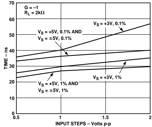
Figure 19. Settling Time vs. Input Step
