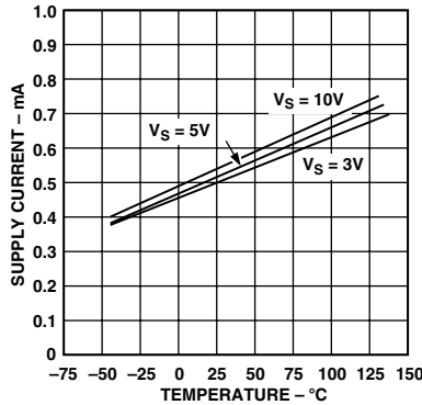
Figure 11. Supply Current/Amplifier vs. Temperature
