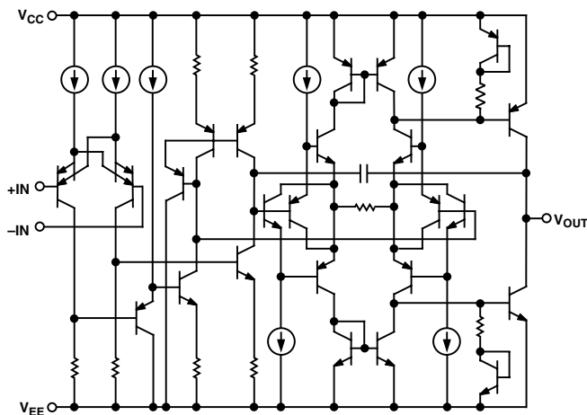
Figure 27. Simplified Schematic
