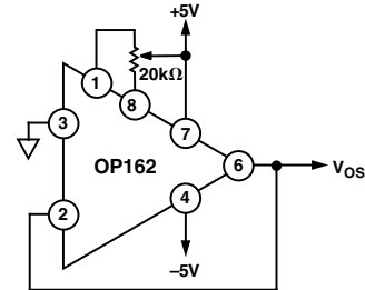
Figure 28. Schematic Showing Offset Adjustment
