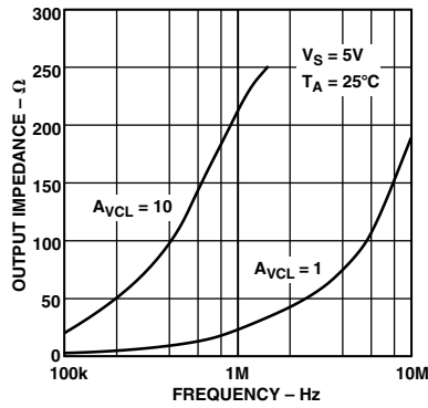
Figure 20. Output Impedance vs. Frequency
