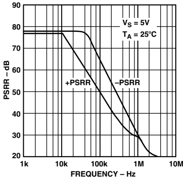
Figure 22. PSRR vs. Frequency
