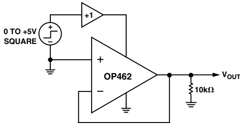
Figure 33. Test Circuit for Power On Settling Time
