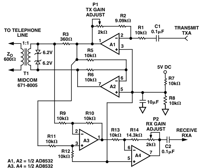
Figure 44. A Single-Supply Direct Access Arrangement for Modems
