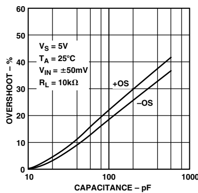
Figure 17. Small-Signal Overshoot vs. Capacitance
