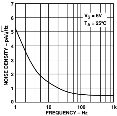
Figure 19. Current Noise Density vs. Frequency
