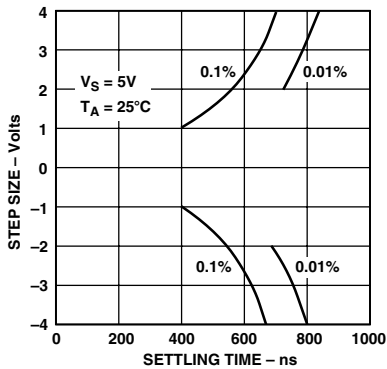
Figure 16. Settling Time vs. Step Size
