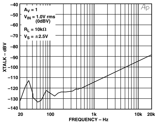
Figure 39. Crosstalk vs. Frequency Graph
