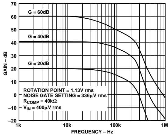
Figure 10b. GBW Curves vs. VCA Gain
