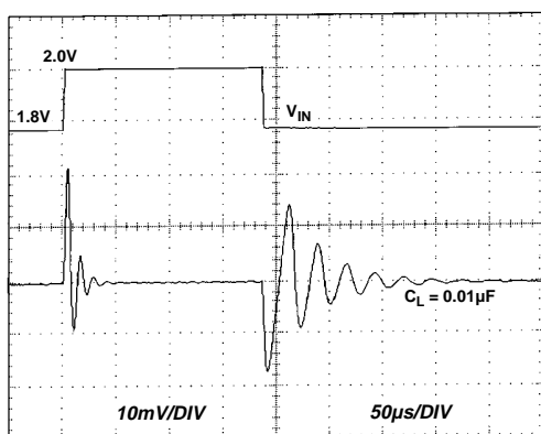
Figure 17. Transient Response with Capacitive Load
