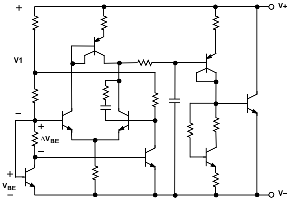
Figure 6. Schematic Diagram
