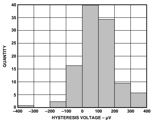
Figure 10. Reverse Voltage Hysteresis Distribution
