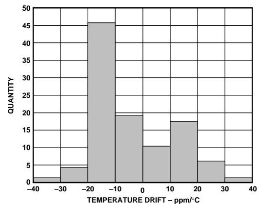
Reverse Voltage Temperature Drift Distribution
