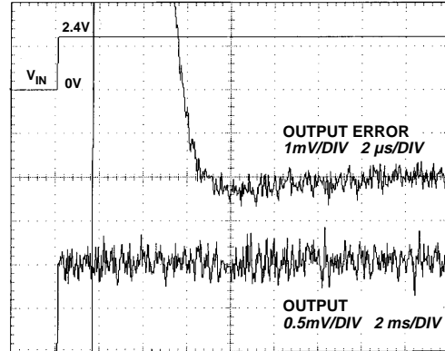
Figure 15. Turn-On Settling
