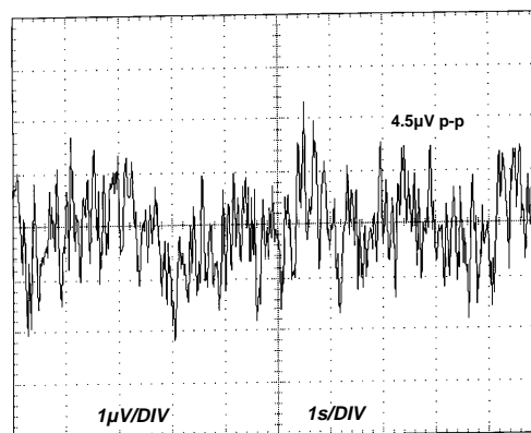
Figure 12. 0.1 Hz–10 Hz Voltage Noise
