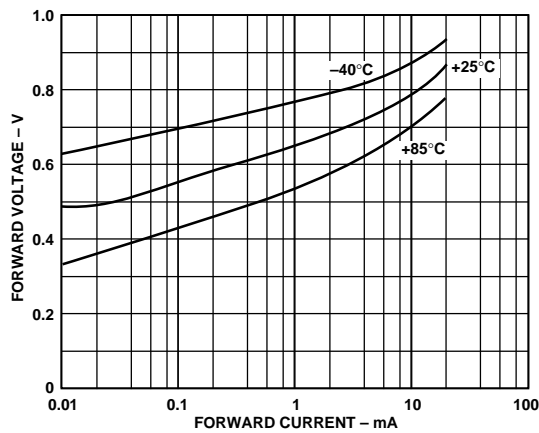
Figure 5. Forward Voltage vs. Forward Current
