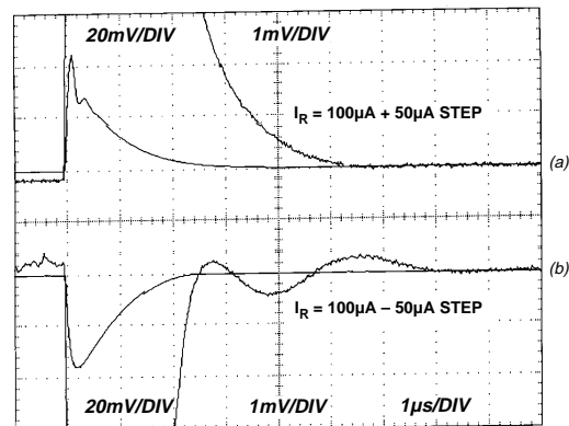
Figure 16. Transient Settling
