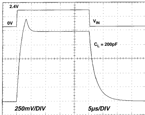
Figure 14a. Response Time
