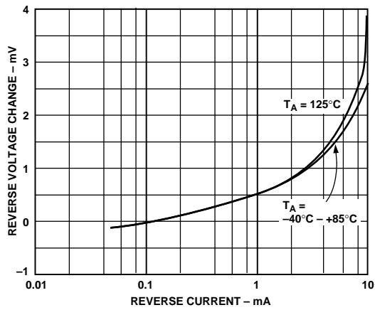
Figure 2. Output Voltage Error vs. Reverse Current
