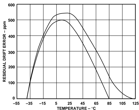
Figure 9. Residual Drift Error
