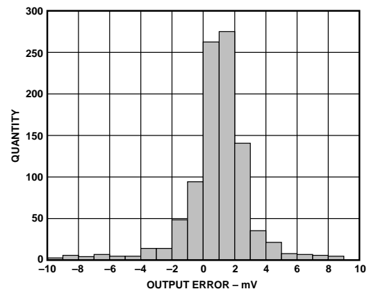
Reverse Voltage Error Distribution
