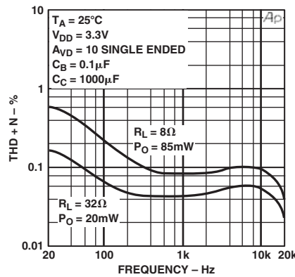
TPC 23. THD+N vs. Frequency
