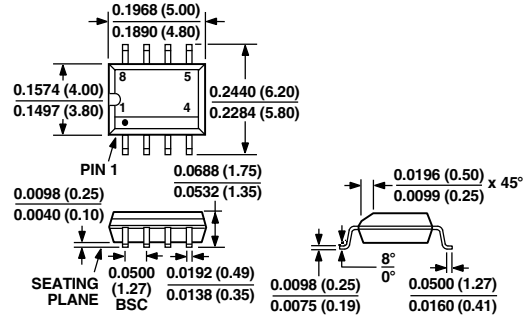
8-Lead SOIC (SO-8)
