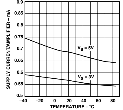
Figure 25. Supply Current per Amplifier vs. Temperature
