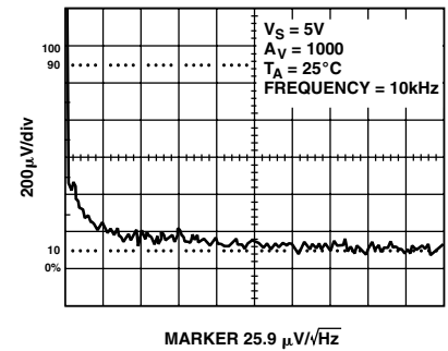
Figure 16. Voltage Noise Density vs. Frequency
