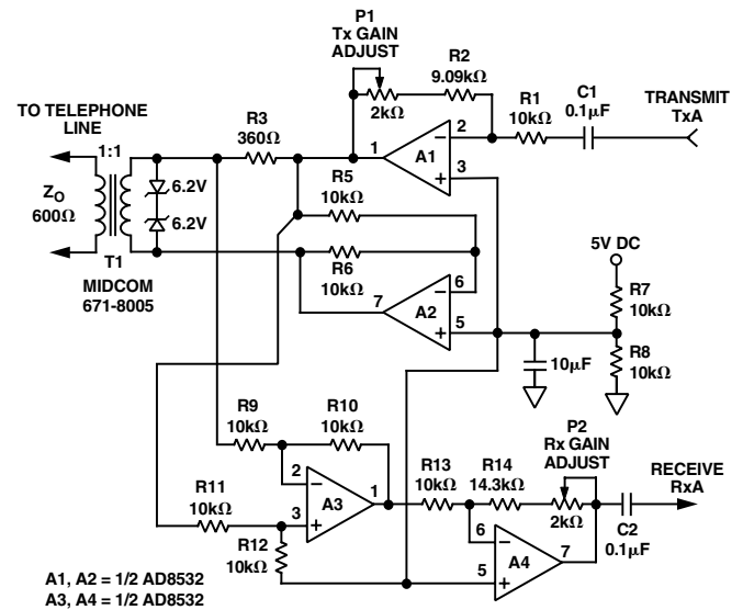
Figure 42. A Single-Supply Direct Access Arrangement for Modems
