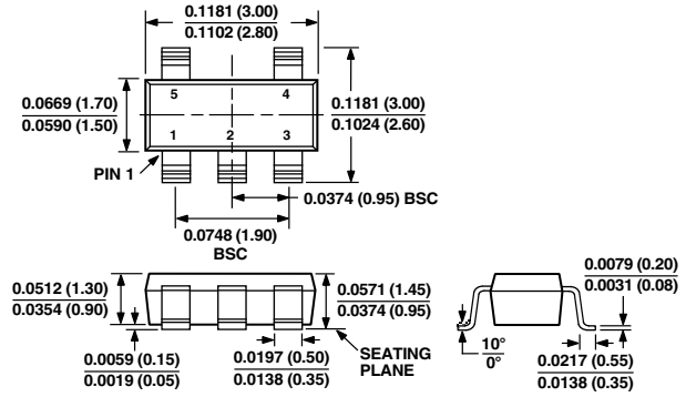
5-Lead SOT-23 (RT-5)
