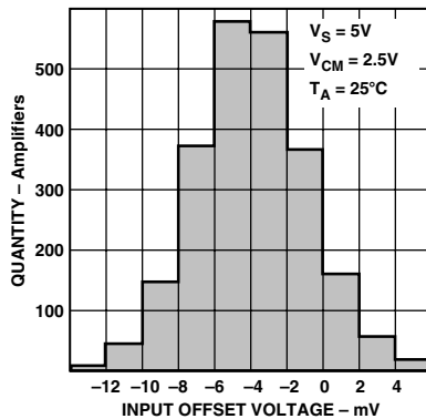
Figure 3. Input Offset Voltage Distribution
