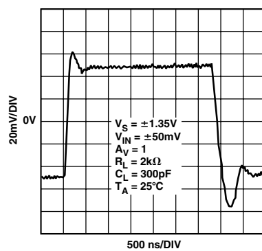
Figure 27. Small Signal Transient Response
