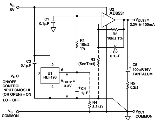
Figure 38. A High Output Current Reference/Regulator
