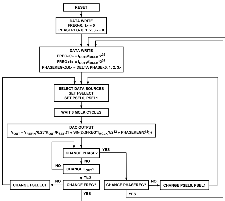
Figure 22. Flow Chart for AD9831 Initialization and Operation
