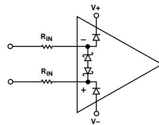
Figure 28. Using Resistors for Input Overcurrent Protection
