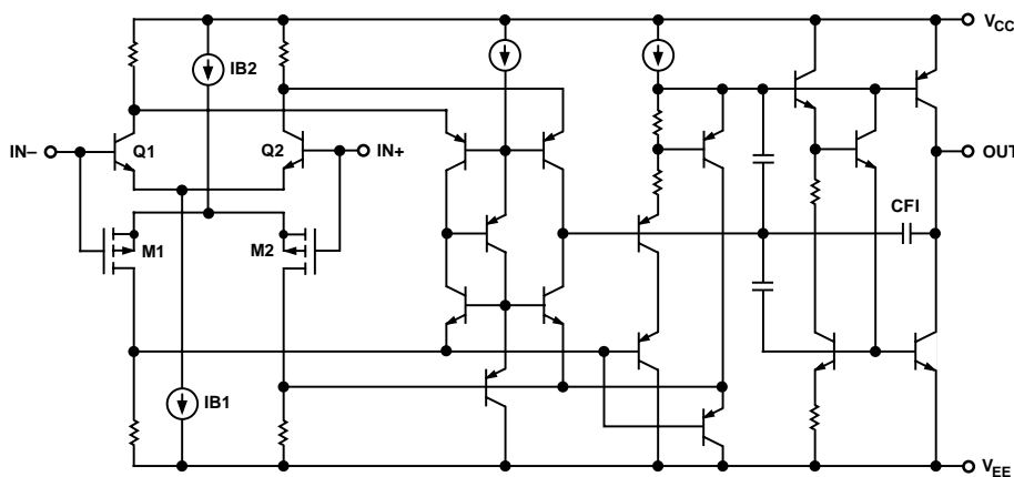
Figure 27. Simplified Schematic
