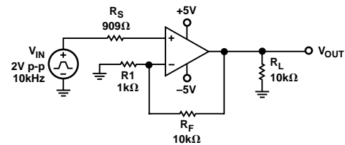
Figure 34. Overload Recovery Time Test Circuit
