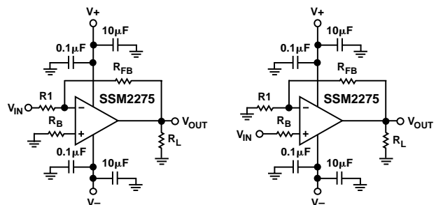
Figure 30. Basic Inverting and Noninverting Amplifiers
