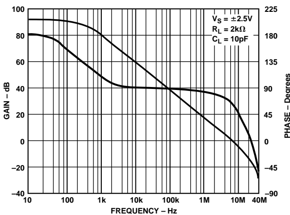
Figure 1. Phase/Gain vs. Frequency
