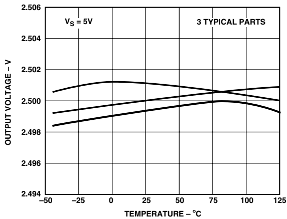
TPC 2. ADR291 V_{OUT} vs. Temperature
