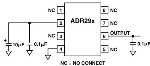
Figure 2. Basic Voltage Reference Configuration
