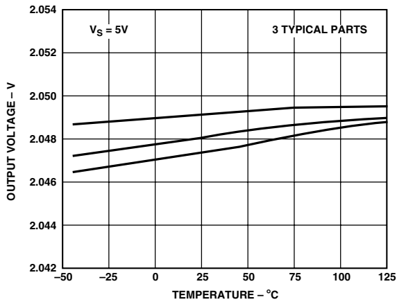
TPC 1. ADR290 V_{OUT} vs. Temperature
