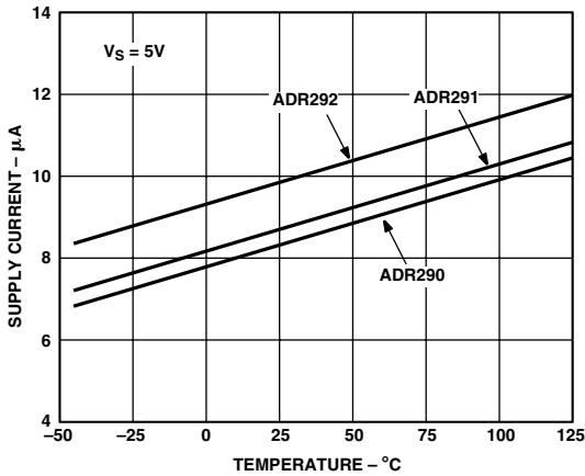
TPC 7. ADR290/ADR291/ADR292 Supply Current vs. Temperature
