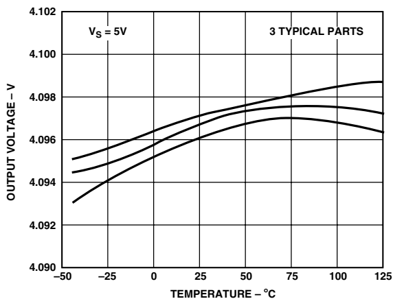
TPC 3. ADR292 V_{OUT} vs. Temperature
