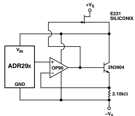
Figure 5. High Voltage Floating Current Source
