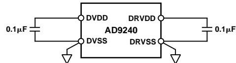
Figure 51. Digital Supply Decoupling
