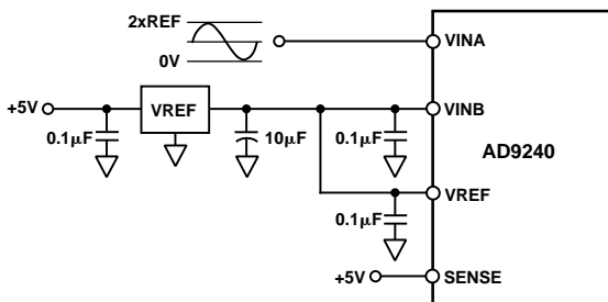
Figure 43. Input Range = 0\text{ V} to 2 \times V_{REF}
