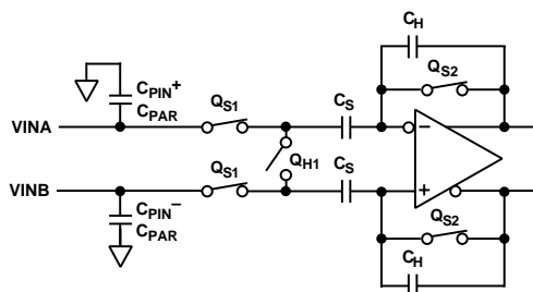
Figure 24. Simplified Input Circuit
