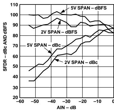
Figure 9. Single Tone SFDR ( f_{IN} = 5.0 MHz, V_{CM} = 2.5 V)
