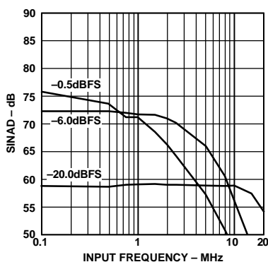
Figure 17. SINAD vs. Input Frequency (Input Span = 5 V, V CM = 2.5 V)
