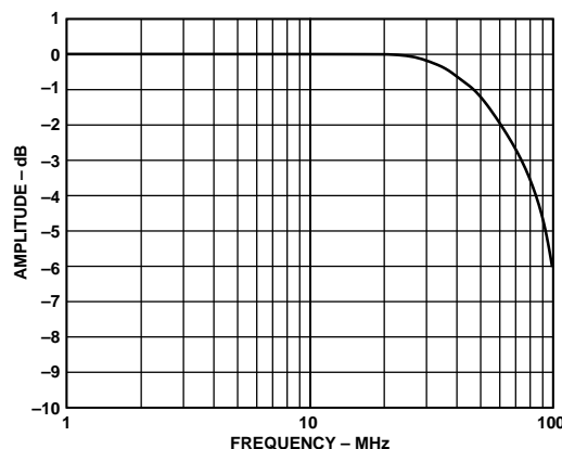
Figure 25. Full-Power Bandwidth
