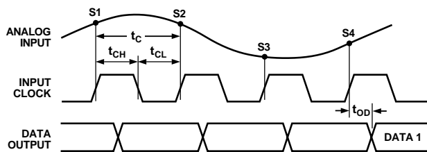
Figure 1. Timing Diagram
