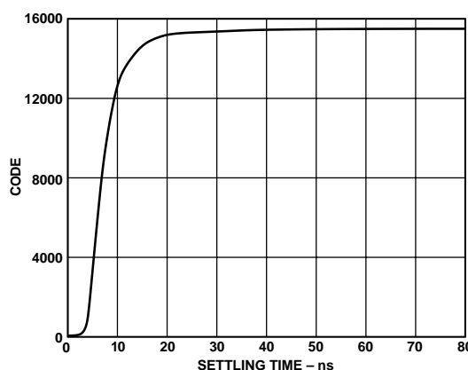
Figure 26. Settling Time
