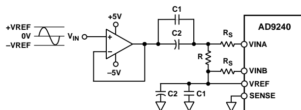
Figure 37. AC-Coupled Input
