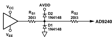
Figure 31. Simple Clamping Circuit
